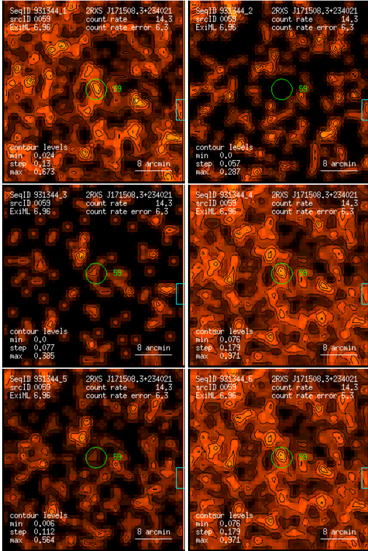
Figure 59: RASS 931344: detection 0059: band rate images, Gaussian filter: (1) PSPC channels 11 – 41, (2) 52 – 90, (3) 91 – 201, (4) 11 – 235, (5) 52 – 201, (6) 11 – 201. Broad band rates in counts/ks. Band rate contour levels in counts/ks/arcmin 2 .
