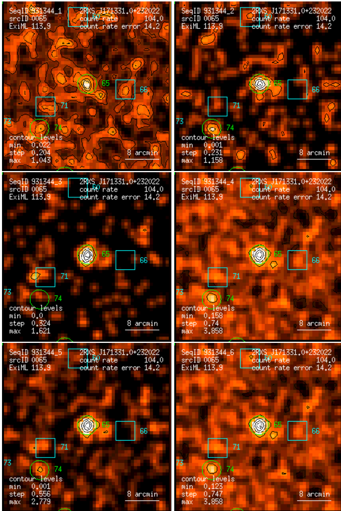
Figure 65: RASS 931344: detection 0065: band rate images, Gaussian filter: (1) PSPC channels 11 – 41, (2) 52 – 90, (3) 91 – 201, (4) 11 – 235, (5) 52 – 201, (6) 11 – 201. Broad band rates in counts/ks. Band rate contour levels in counts/ks/arcmin 2 .
