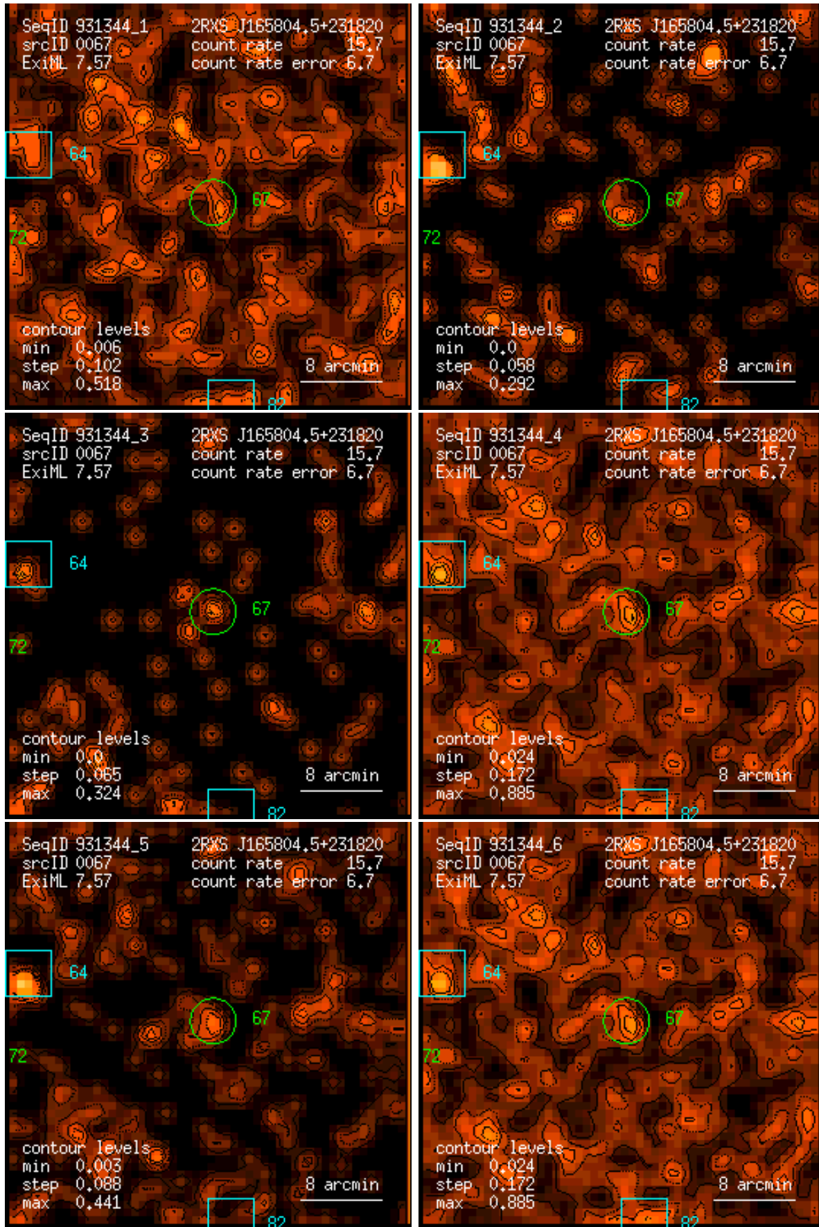
Figure 67: RASS 931344: detection 0067: band rate images, Gaussian filter: (1) PSPC channels 11 – 41, (2) 52 – 90, (3) 91 – 201, (4) 11 – 235, (5) 52 – 201, (6) 11 – 201. Broad band rates in counts/ks. Band rate contour levels in counts/ks/arcmin 2 .
