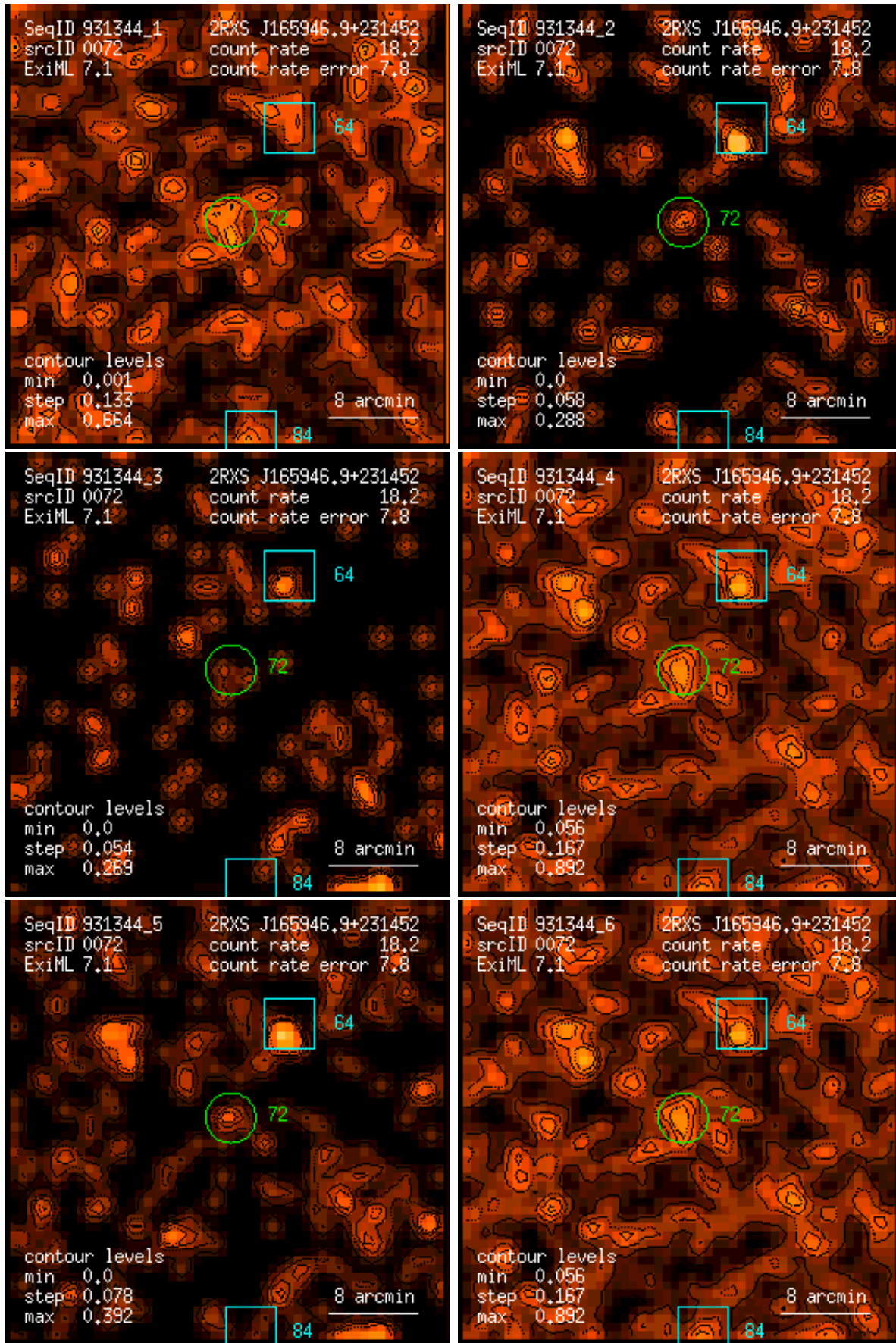
Figure 72: RASS 931344: detection 0072: band rate images, Gaussian filter: (1) PSPC channels 11 – 41, (2) 52 – 90, (3) 91 – 201, (4) 11 – 235, (5) 52 – 201, (6) 11 – 201. Broad band rates in counts/ks. Band rate contour levels in counts/ks/arcmin 2 .
