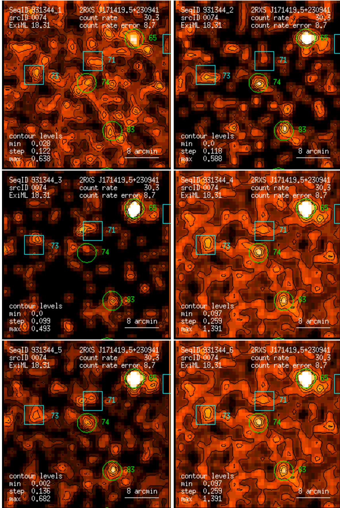
Figure 74: RASS 931344: detection 0074: band rate images, Gaussian filter: (1) PSPC channels 11 – 41, (2) 52 – 90, (3) 91 – 201, (4) 11 – 235, (5) 52 – 201, (6) 11 – 201. Broad band rates in counts/ks. Band rate contour levels in counts/ks/arcmin 2 .
