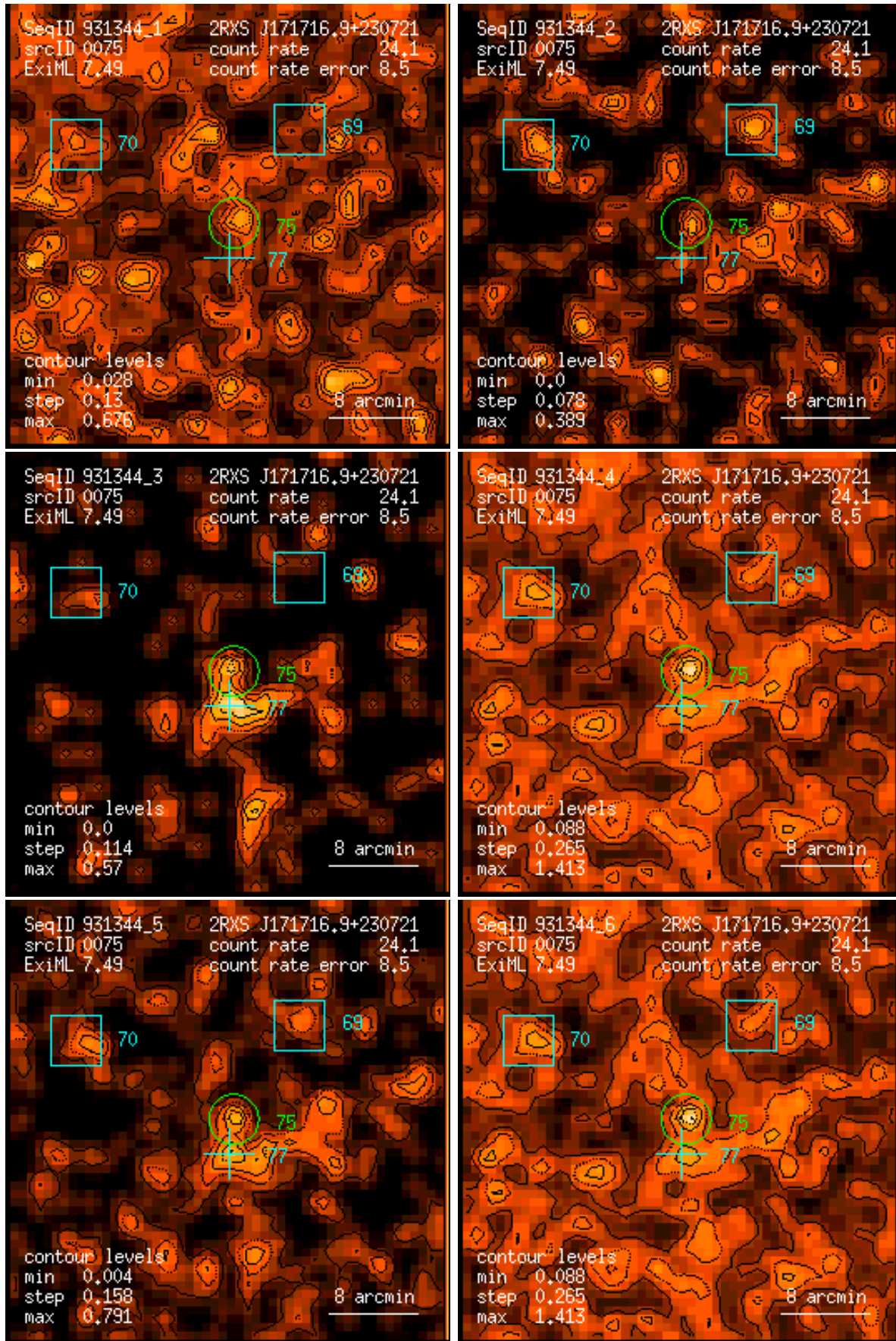
Figure 75: RASS 931344: detection 0075: band rate images, Gaussian filter: (1) PSPC channels 11 – 41, (2) 52 – 90, (3) 91 – 201, (4) 11 – 235, (5) 52 – 201, (6) 11 – 201. Broad band rates in counts/ks. Band rate contour levels in counts/ks/arcmin 2 .
