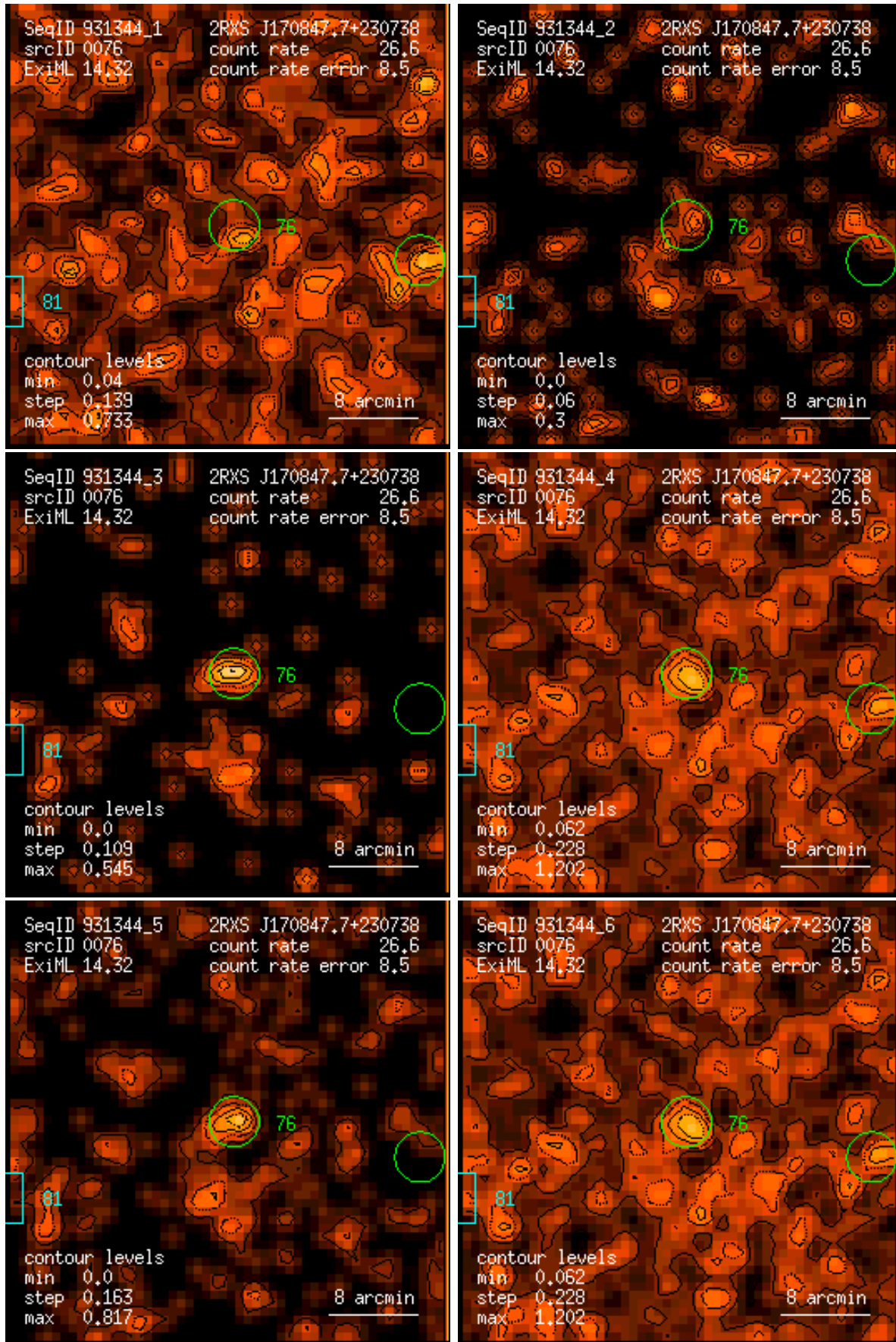
Figure 76: RASS 931344: detection 0076: band rate images, Gaussian filter: (1) PSPC channels 11 – 41, (2) 52 – 90, (3) 91 – 201, (4) 11 – 235, (5) 52 – 201, (6) 11 – 201. Broad band rates in counts/ks. Band rate contour levels in counts/ks/arcmin 2 .
