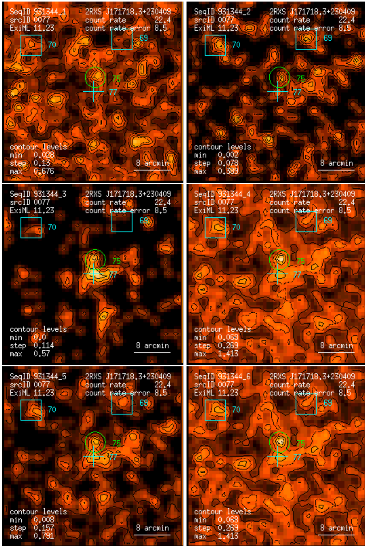
Figure 77: RASS 931344: detection 0077: band rate images, Gaussian filter: (1) PSPC channels 11 – 41, (2) 52 – 90, (3) 91 – 201, (4) 11 – 235, (5) 52 – 201, (6) 11 – 201. Broad band rates in counts/ks. Band rate contour levels in counts/ks/arcmin 2 .
