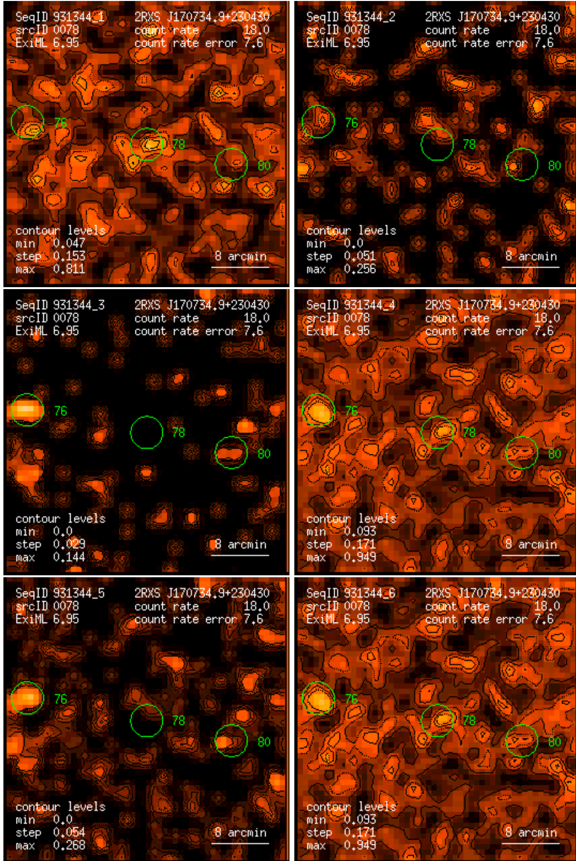
Figure 78: RASS 931344: detection 0078: band rate images, Gaussian filter: (1) PSPC channels 11 – 41, (2) 52 – 90, (3) 91 – 201, (4) 11 – 235, (5) 52 – 201, (6) 11 – 201. Broad band rates in counts/ks. Band rate contour levels in counts/ks/arcmin 2 .
