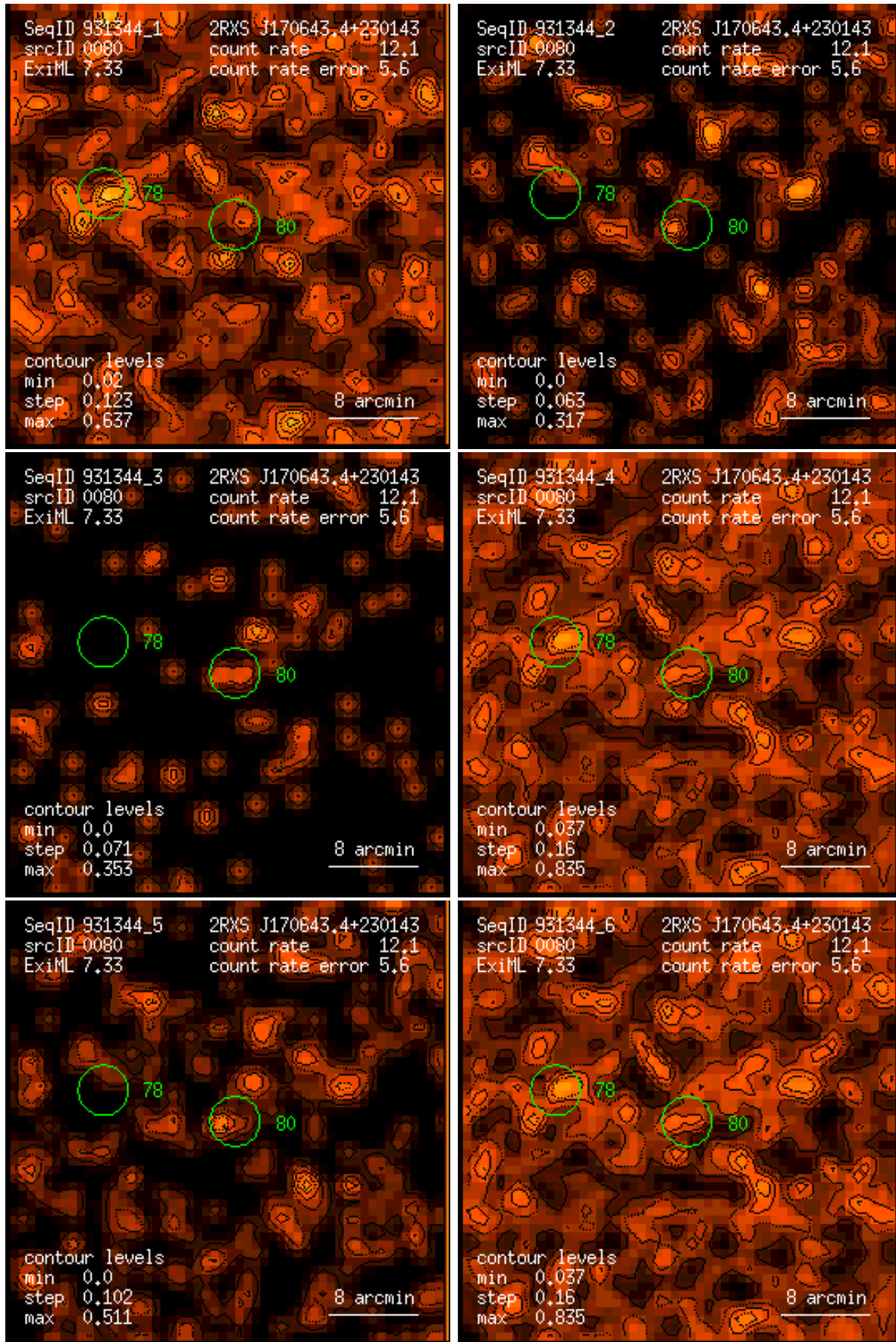
Figure 80: RASS 931344: detection 0080: band rate images, Gaussian filter: (1) PSPC channels 11 – 41, (2) 52 – 90, (3) 91 – 201, (4) 11 – 235, (5) 52 – 201, (6) 11 – 201. Broad band rates in counts/ks. Band rate contour levels in counts/ks/arcmin 2 .
