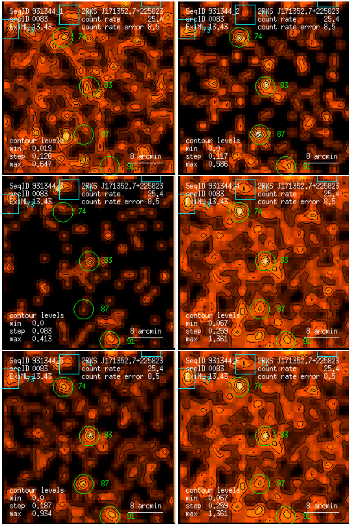
Figure 83: RASS 931344: detection 0083: band rate images, Gaussian filter: (1) PSPC channels 11 – 41, (2) 52 – 90, (3) 91 – 201, (4) 11 – 235, (5) 52 – 201, (6) 11 – 201. Broad band rates in counts/ks. Band rate contour levels in counts/ks/arcmin 2 .
