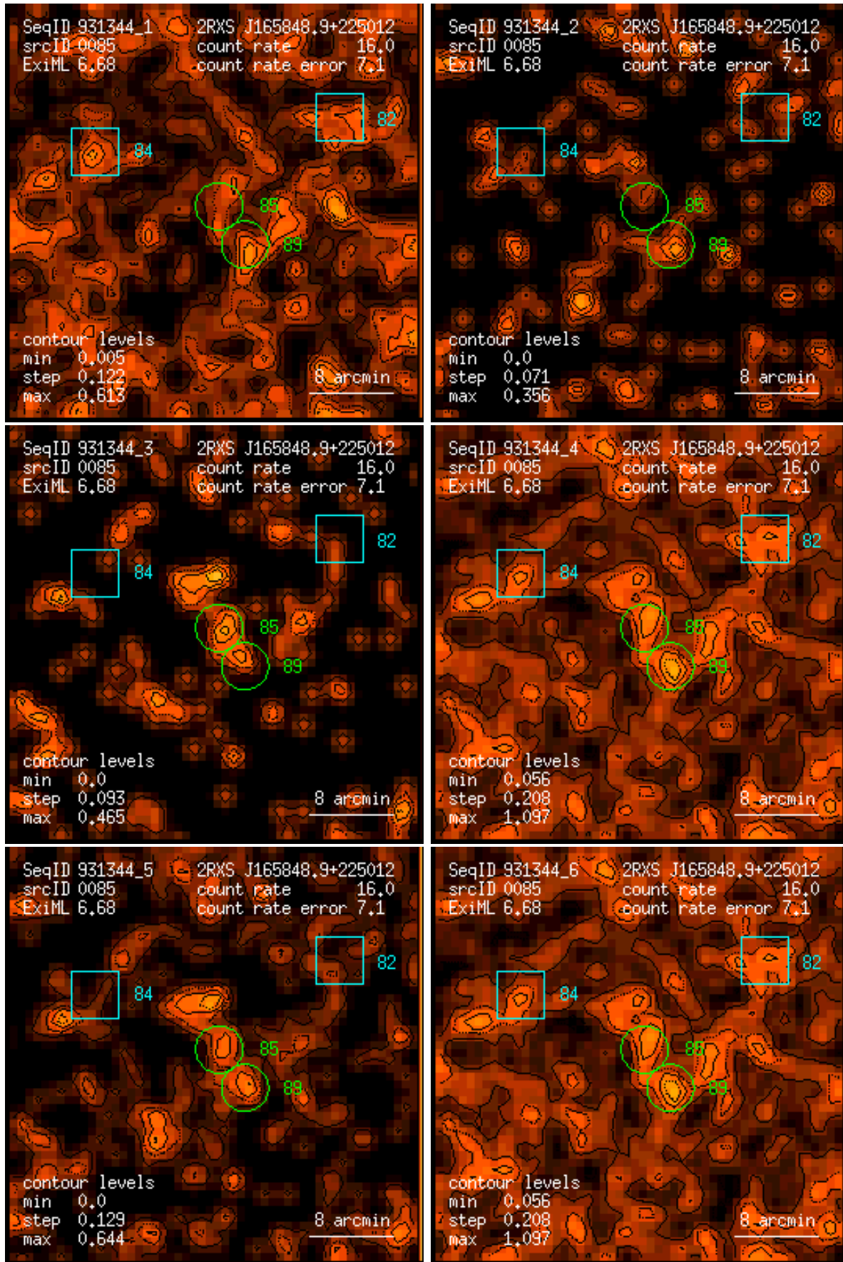
Figure 85: RASS 931344: detection 0085: band rate images, Gaussian filter: (1) PSPC channels 11 – 41, (2) 52 – 90, (3) 91 – 201, (4) 11 – 235, (5) 52 – 201, (6) 11 – 201. Broad band rates in counts/ks. Band rate contour levels in counts/ks/arcmin 2 .
