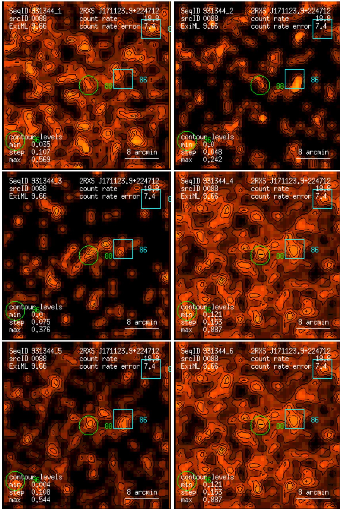
Figure 88: RASS 931344: detection 0088: band rate images, Gaussian filter: (1) PSPC channels 11 – 41, (2) 52 – 90, (3) 91 – 201, (4) 11 – 235, (5) 52 – 201, (6) 11 – 201. Broad band rates in counts/ks. Band rate contour levels in counts/ks/arcmin 2 .
