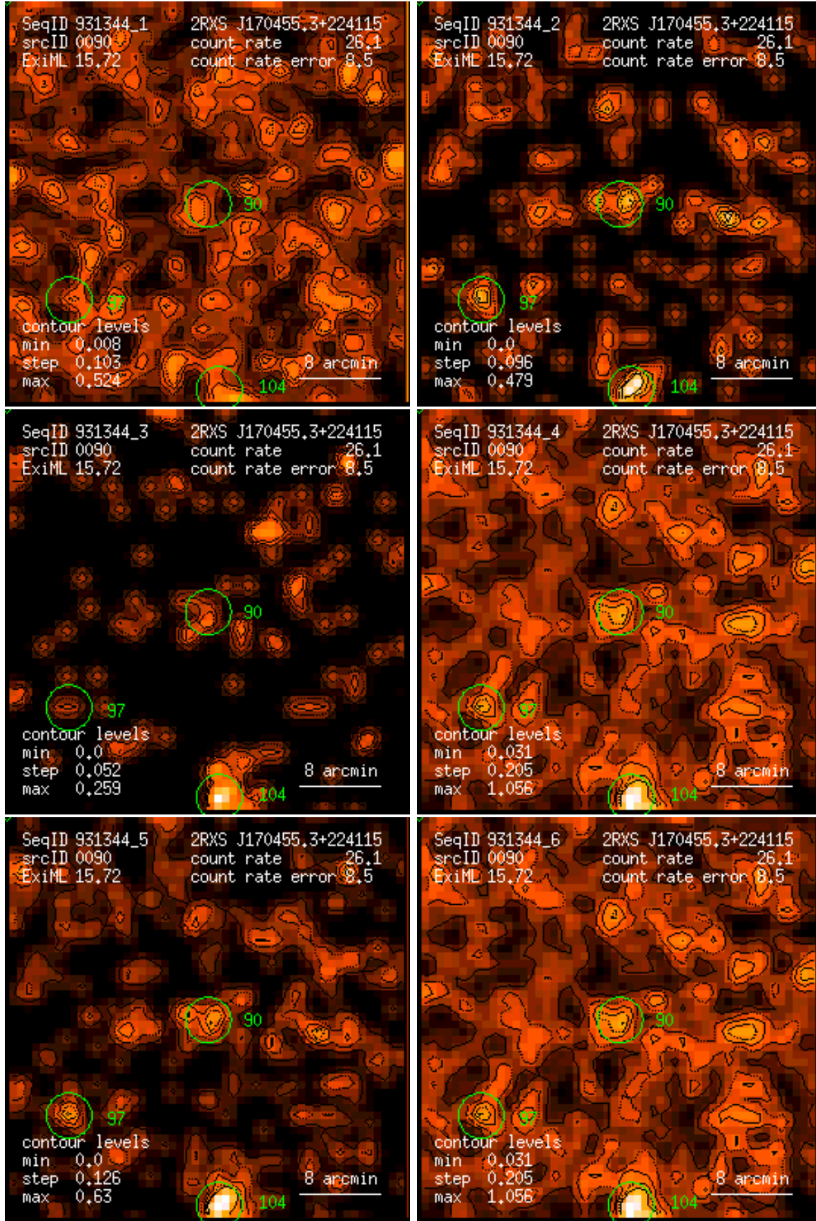
Figure 90: RASS 931344: detection 0090: band rate images, Gaussian filter: (1) PSPC channels 11 – 41, (2) 52 – 90, (3) 91 – 201, (4) 11 – 235, (5) 52 – 201, (6) 11 – 201. Broad band rates in counts/ks. Band rate contour levels in counts/ks/arcmin 2 .
