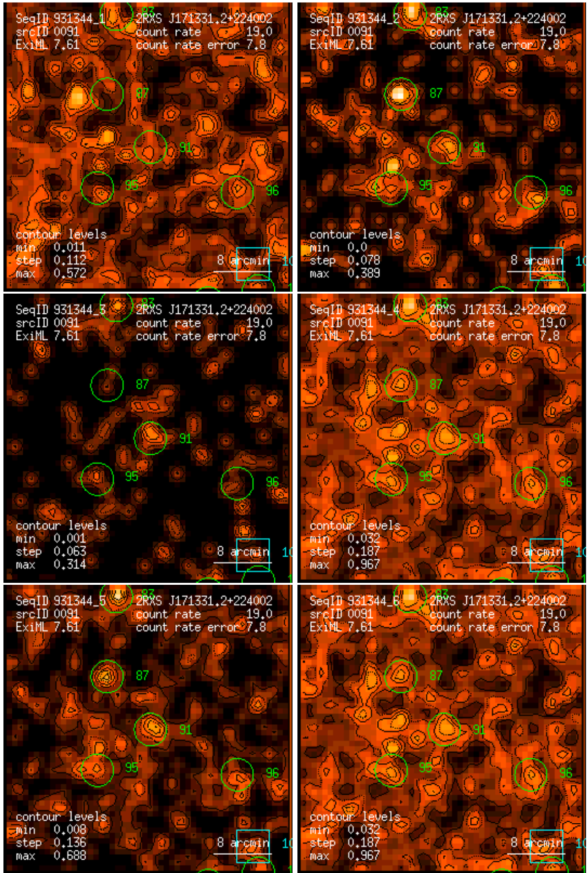
Figure 91: RASS 931344: detection 0091: band rate images, Gaussian filter: (1) PSPC channels 11 – 41, (2) 52 – 90, (3) 91 – 201, (4) 11 – 235, (5) 52 – 201, (6) 11 – 201. Broad band rates in counts/ks. Band rate contour levels in counts/ks/arcmin 2 .
