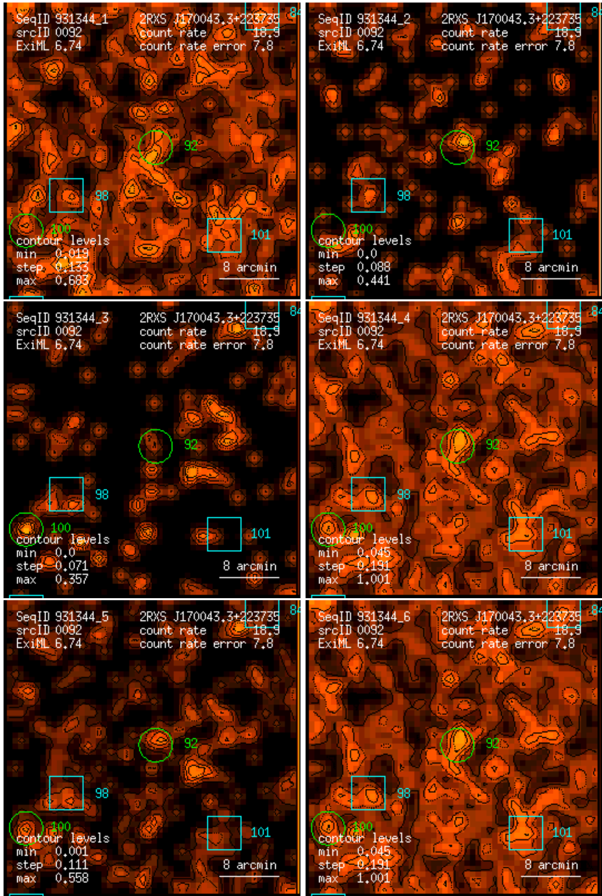
Figure 92: RASS 931344: detection 0092: band rate images, Gaussian filter: (1) PSPC channels 11 – 41, (2) 52 – 90, (3) 91 – 201, (4) 11 – 235, (5) 52 – 201, (6) 11 – 201. Broad band rates in counts/ks. Band rate contour levels in counts/ks/arcmin 2 .
