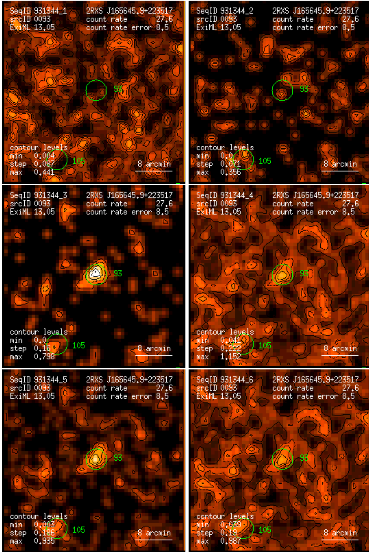
Figure 93: RASS 931344: detection 0093: band rate images, Gaussian filter: (1) PSPC channels 11 – 41, (2) 52 – 90, (3) 91 – 201, (4) 11 – 235, (5) 52 – 201, (6) 11 – 201. Broad band rates in counts/ks. Band rate contour levels in counts/ks/arcmin 2 .
