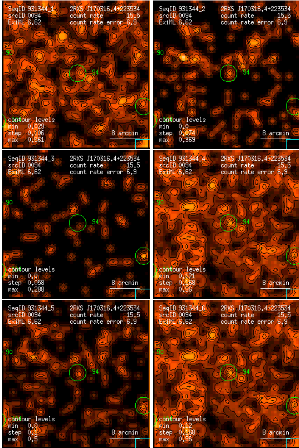
Figure 94: RASS 931344: detection 0094: band rate images, Gaussian filter: (1) PSPC channels 11 – 41, (2) 52 – 90, (3) 91 – 201, (4) 11 – 235, (5) 52 – 201, (6) 11 – 201. Broad band rates in counts/ks. Band rate contour levels in counts/ks/arcmin 2 .
