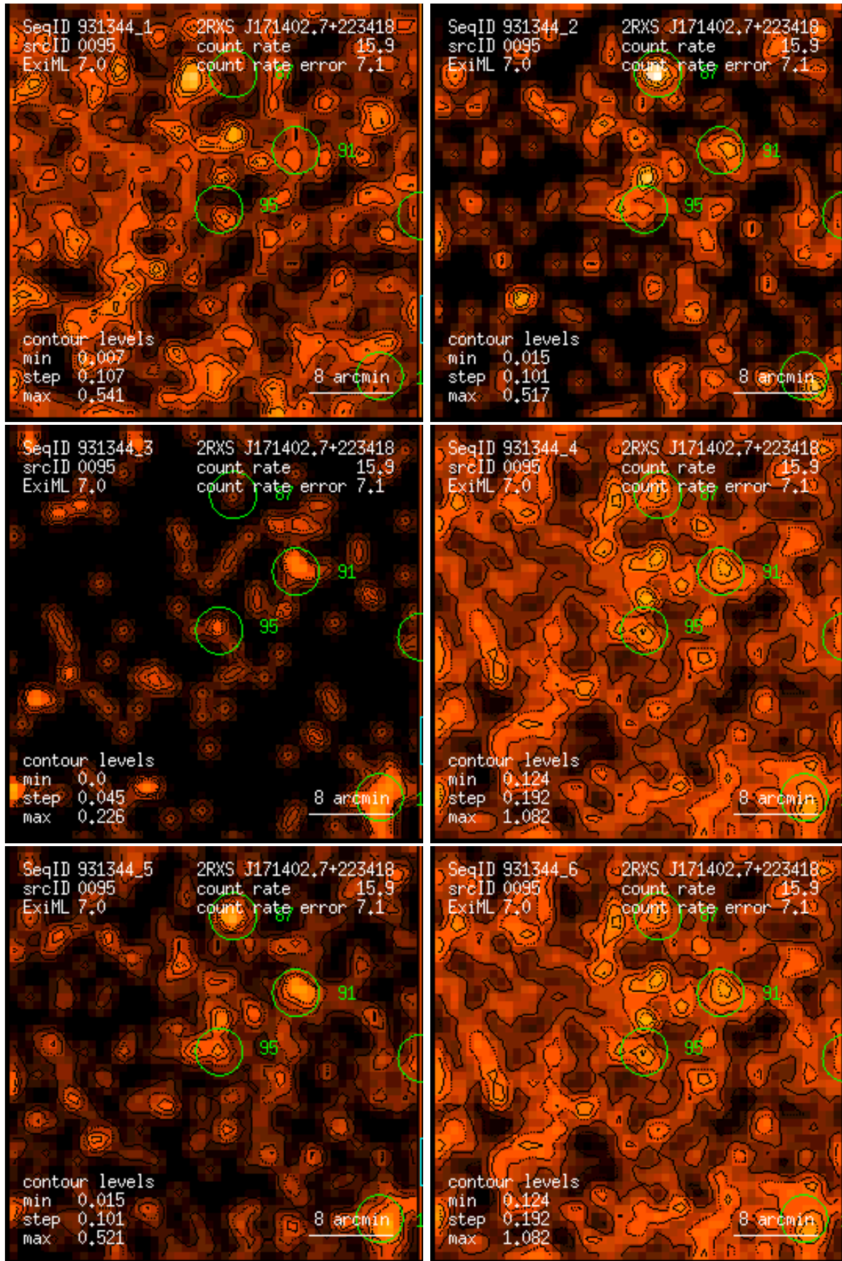
Figure 95: RASS 931344: detection 0095: band rate images, Gaussian filter: (1) PSPC channels 11 – 41, (2) 52 – 90, (3) 91 – 201, (4) 11 – 235, (5) 52 – 201, (6) 11 – 201. Broad band rates in counts/ks. Band rate contour levels in counts/ks/arcmin 2 .
