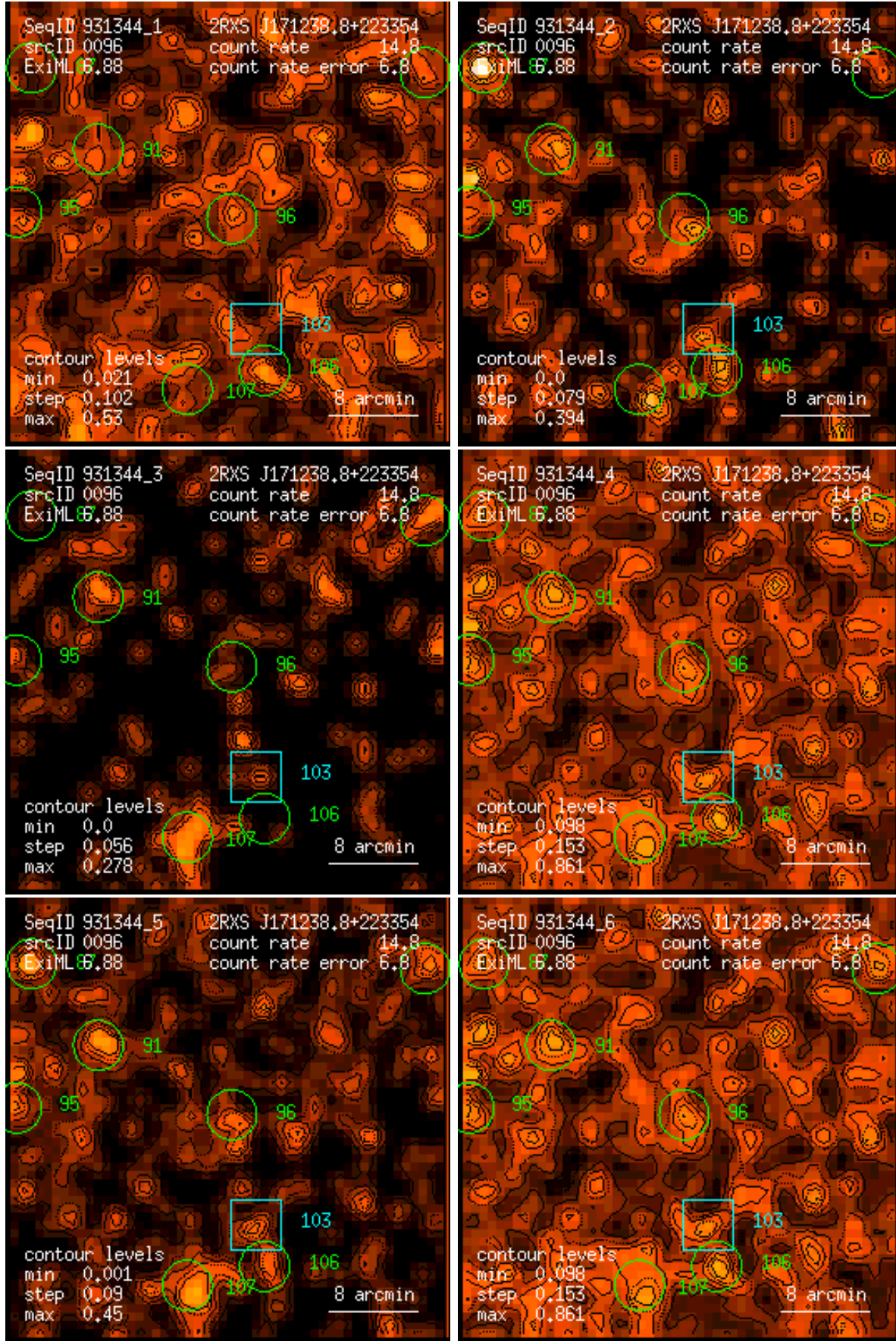
Figure 96: RASS 931344: detection 0096: band rate images, Gaussian filter: (1) PSPC channels 11 – 41, (2) 52 – 90, (3) 91 – 201, (4) 11 – 235, (5) 52 – 201, (6) 11 – 201. Broad band rates in counts/ks. Band rate contour levels in counts/ks/arcmin 2 .
