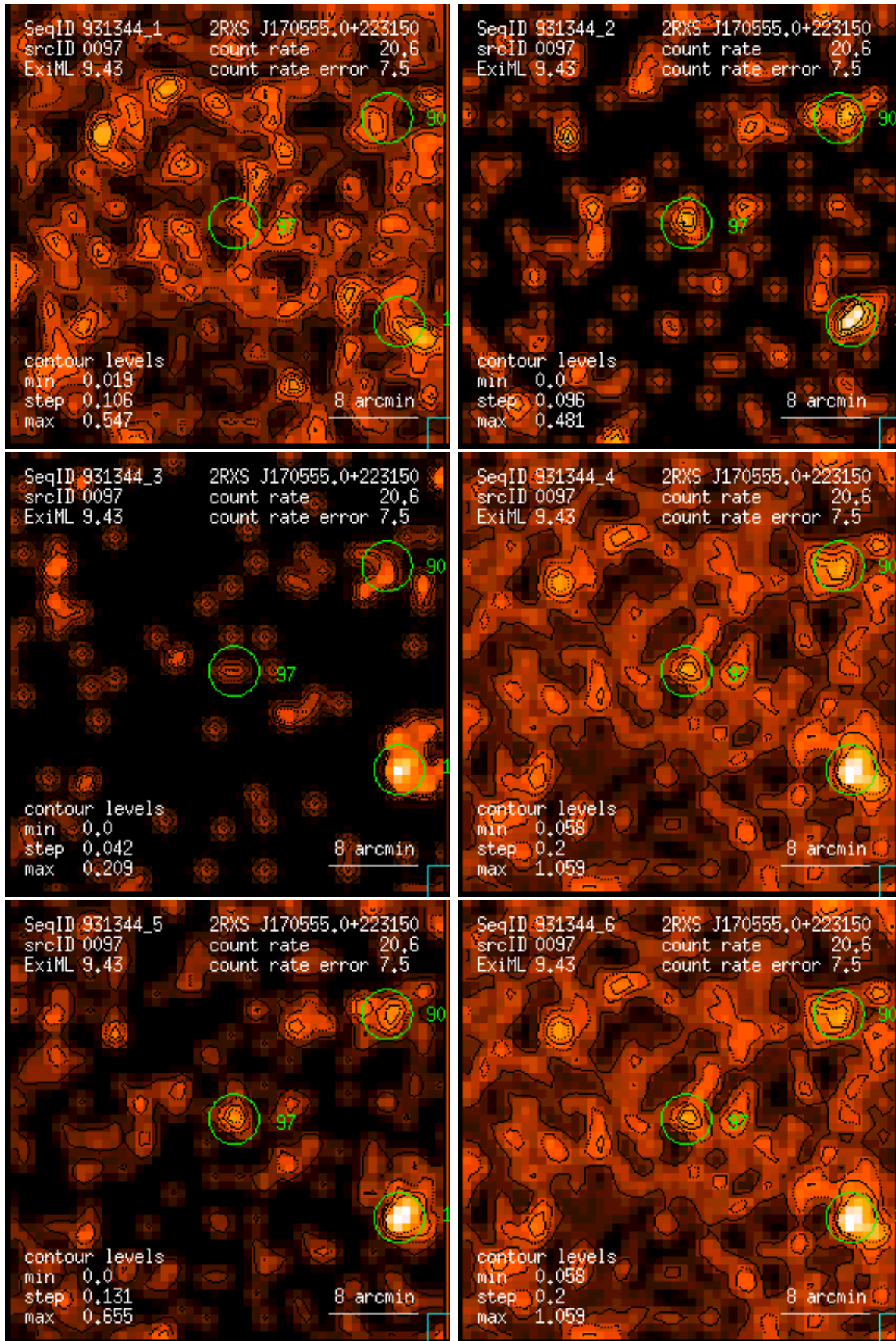
Figure 97: RASS 931344: detection 0097: band rate images, Gaussian filter: (1) PSPC channels 11 – 41, (2) 52 – 90, (3) 91 – 201, (4) 11 – 235, (5) 52 – 201, (6) 11 – 201. Broad band rates in counts/ks. Band rate contour levels in counts/ks/arcmin 2 .
