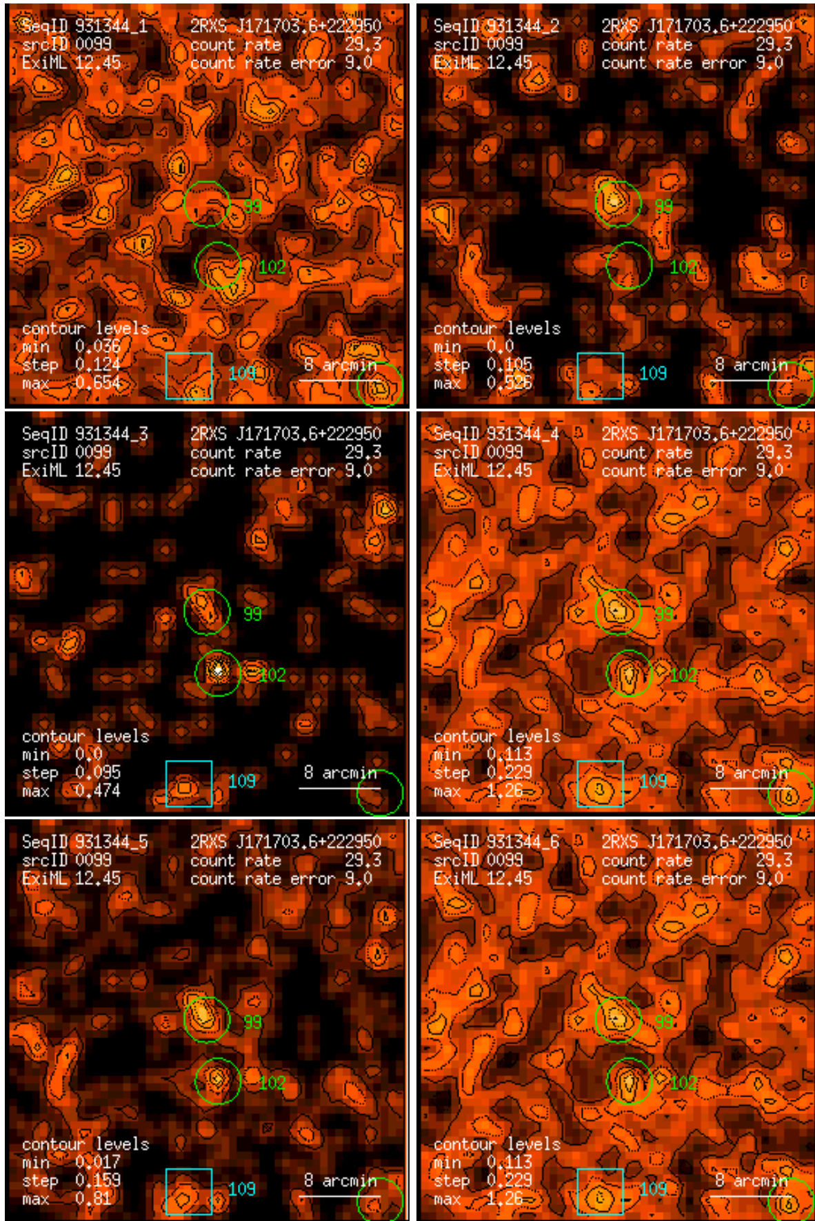
Figure 99: RASS 931344: detection 0099: band rate images, Gaussian filter: (1) PSPC channels 11 – 41, (2) 52 – 90, (3) 91 – 201, (4) 11 – 235, (5) 52 – 201, (6) 11 – 201. Broad band rates in counts/ks. Band rate contour levels in counts/ks/arcmin 2 .
