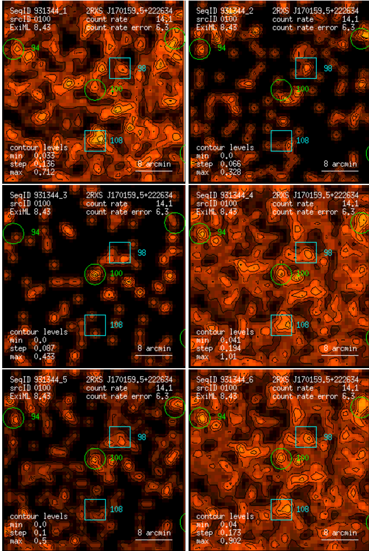
Figure 100: RASS 931344: detection 0100: band rate images, Gaussian filter: (1) PSPC channels 11 – 41, (2) 52 – 90, (3) 91 – 201, (4) 11 – 235, (5) 52 – 201, (6) 11 – 201. Broad band rates in counts/ks. Band rate contour levels in counts/ks/arcmin 2 .
