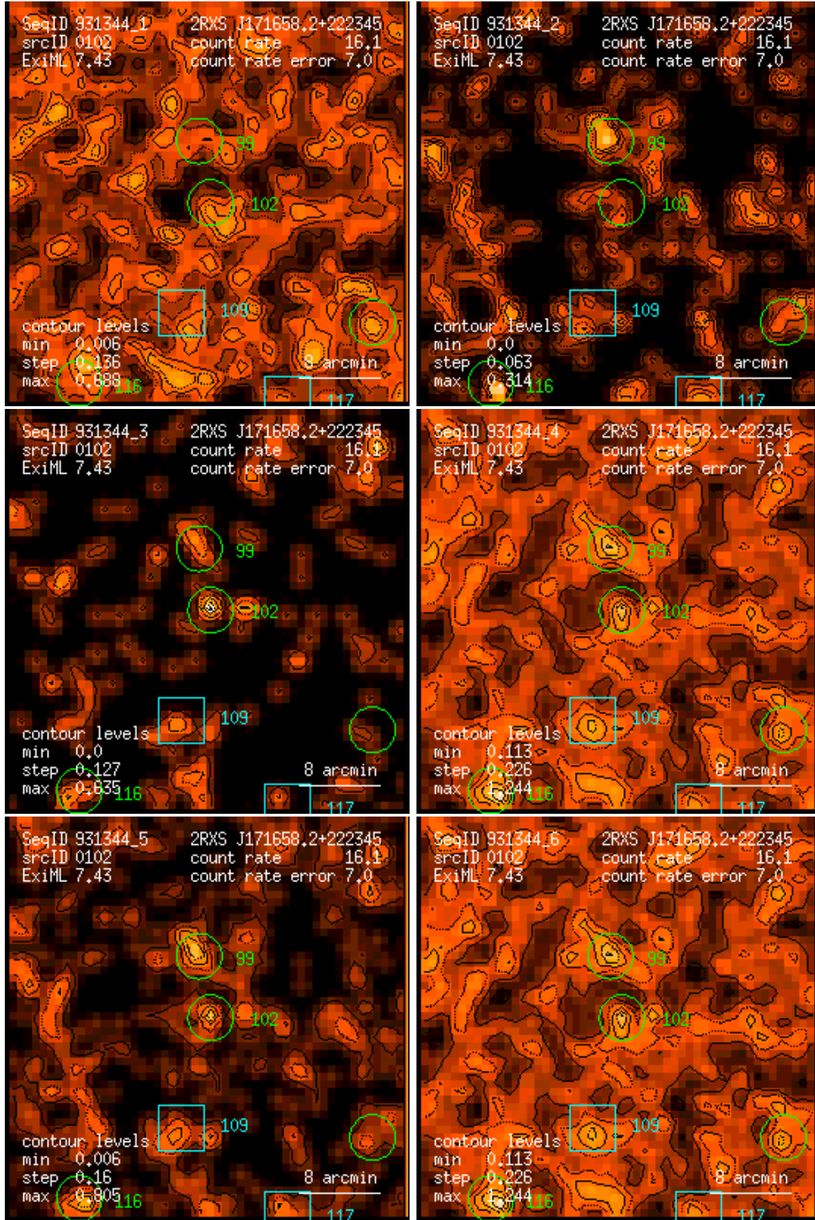
Figure 102: RASS 931344: detection 0102: band rate images, Gaussian filter: (1) PSPC channels 11 – 41, (2) 52 – 90, (3) 91 – 201, (4) 11 – 235, (5) 52 – 201, (6) 11 – 201. Broad band rates in counts/ks. Band rate contour levels in counts/ks/arcmin 2 .
