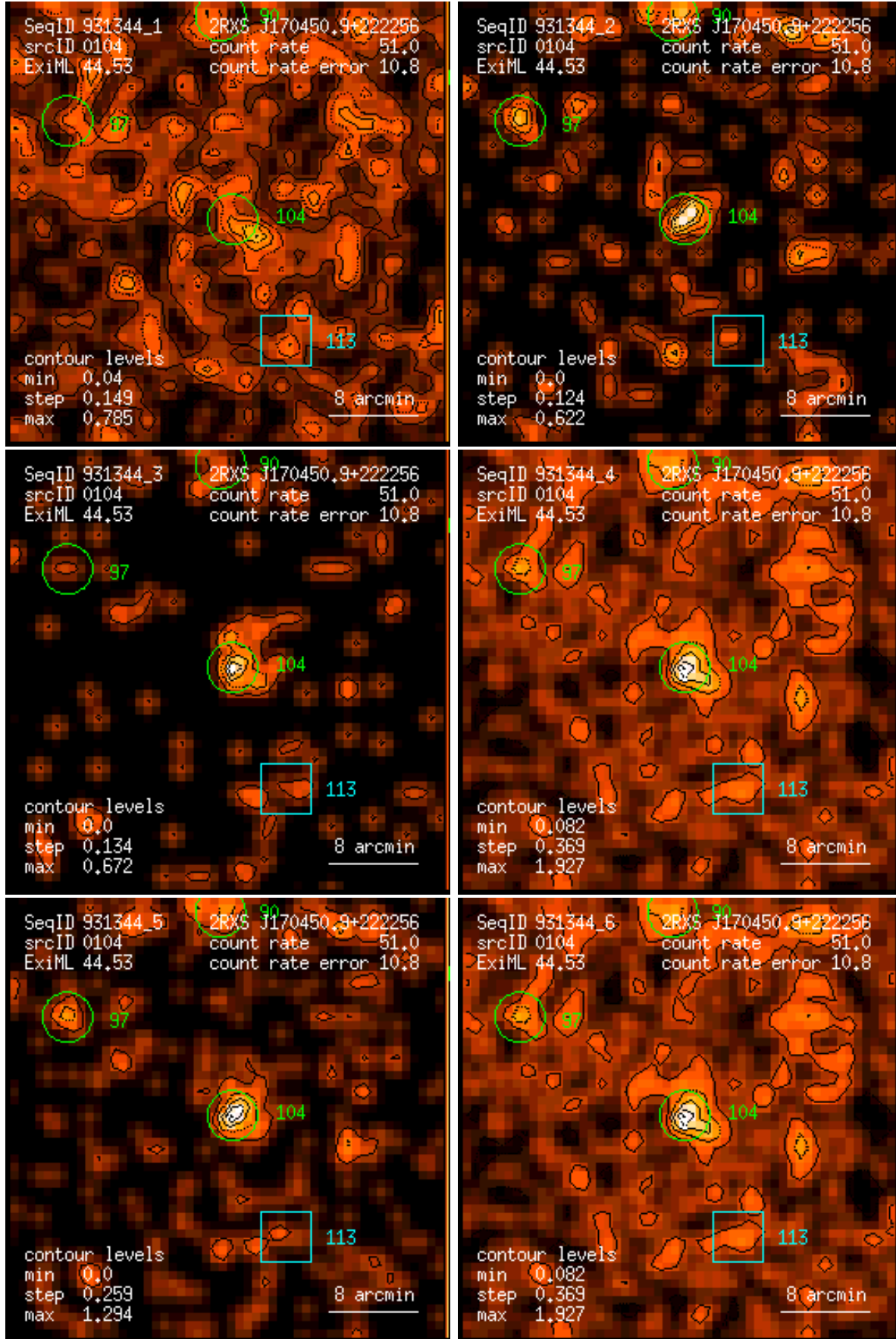
Figure 104: RASS 931344: detection 0104: band rate images, Gaussian filter: (1) PSPC channels 11 – 41, (2) 52 – 90, (3) 91 – 201, (4) 11 – 235, (5) 52 – 201, (6) 11 – 201. Broad band rates in counts/ks. Band rate contour levels in counts/ks/arcmin 2 .
