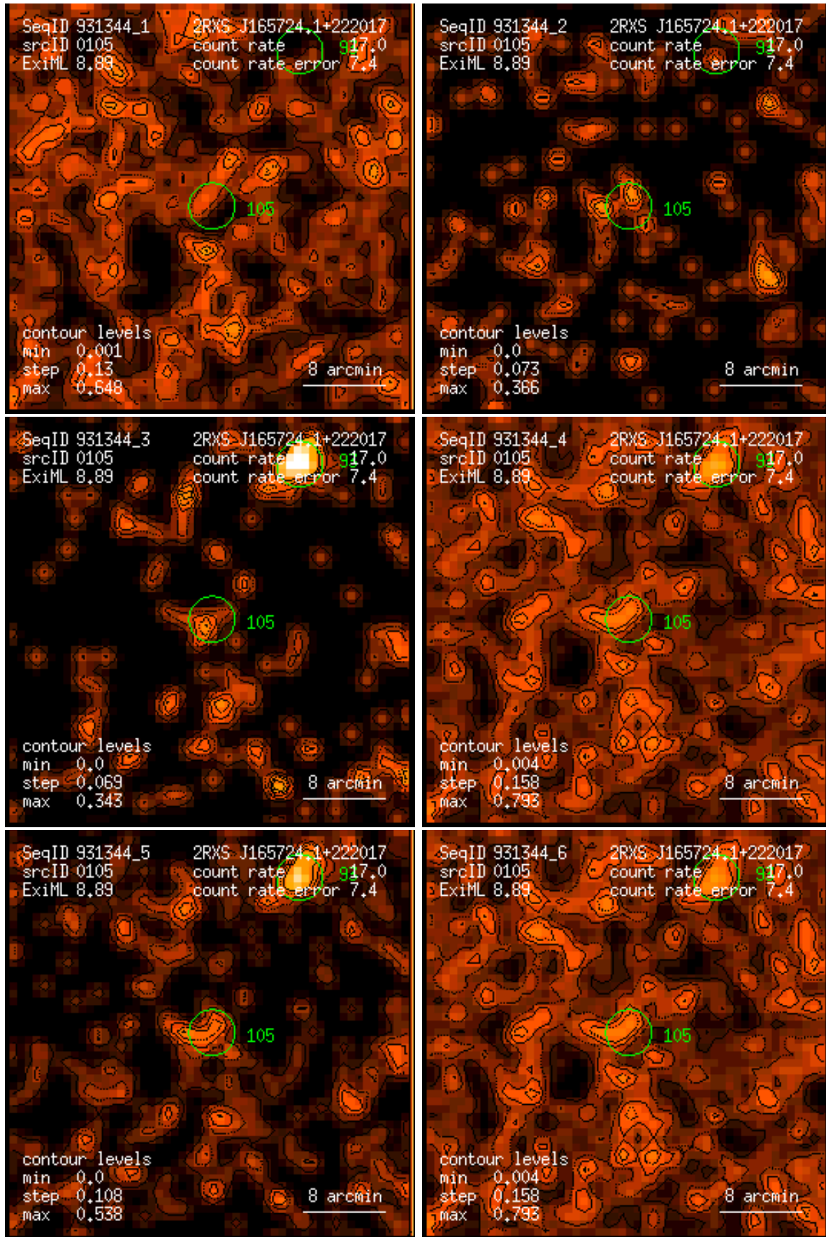
Figure 105: RASS 931344: detection 0105: band rate images, Gaussian filter: (1) PSPC channels 11 – 41, (2) 52 – 90, (3) 91 – 201, (4) 11 – 235, (5) 52 – 201, (6) 11 – 201. Broad band rates in counts/ks. Band rate contour levels in counts/ks/arcmin 2 .
