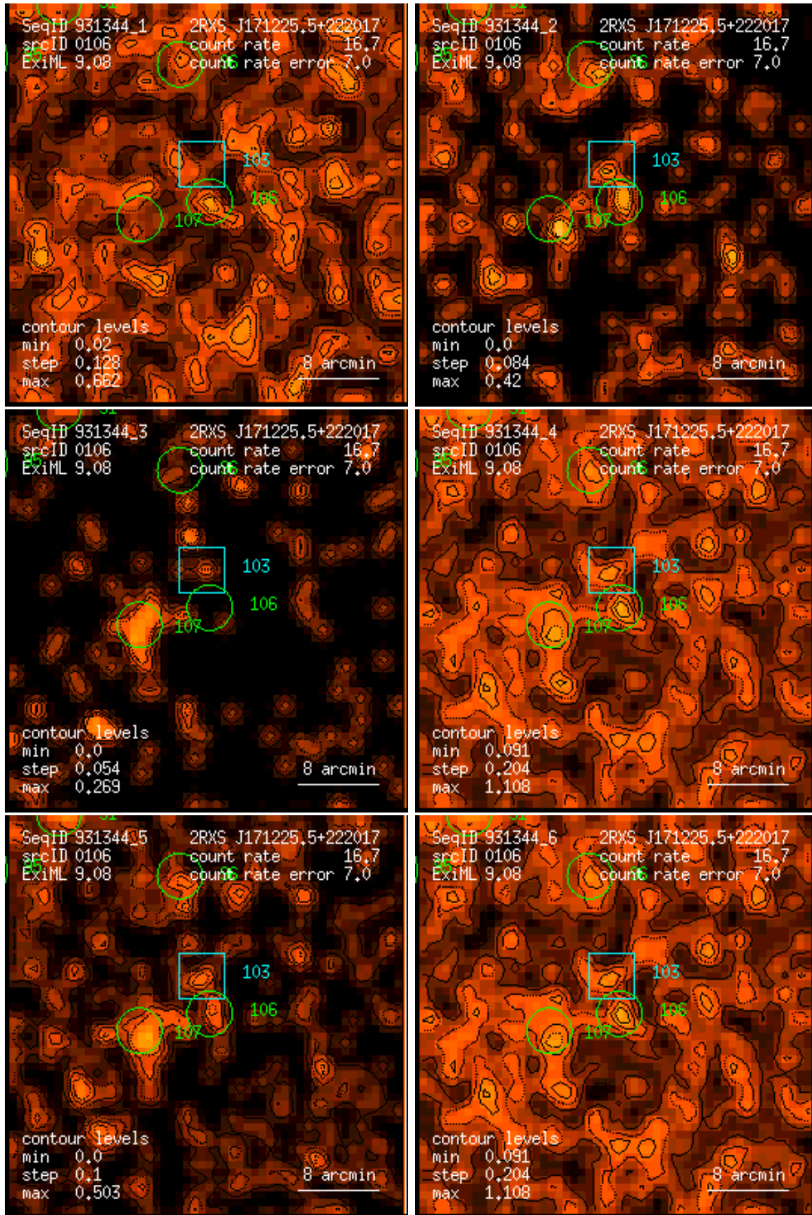
Figure 106: RASS 931344: detection 0106: band rate images, Gaussian filter: (1) PSPC channels 11 – 41, (2) 52 – 90, (3) 91 – 201, (4) 11 – 235, (5) 52 – 201, (6) 11 – 201. Broad band rates in counts/ks. Band rate contour levels in counts/ks/arcmin 2 .
