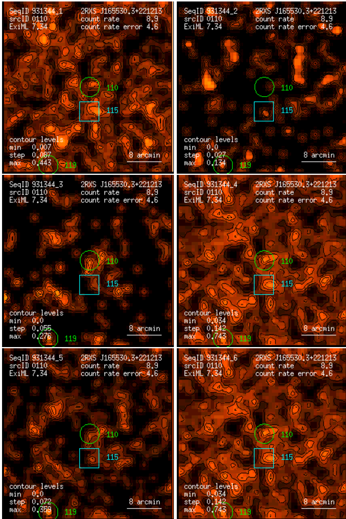
Figure 110: RASS 931344: detection 0110: band rate images, Gaussian filter: (1) PSPC channels 11 – 41, (2) 52 – 90, (3) 91 – 201, (4) 11 – 235, (5) 52 – 201, (6) 11 – 201. Broad band rates in counts/ks. Band rate contour levels in counts/ks/arcmin 2 .
