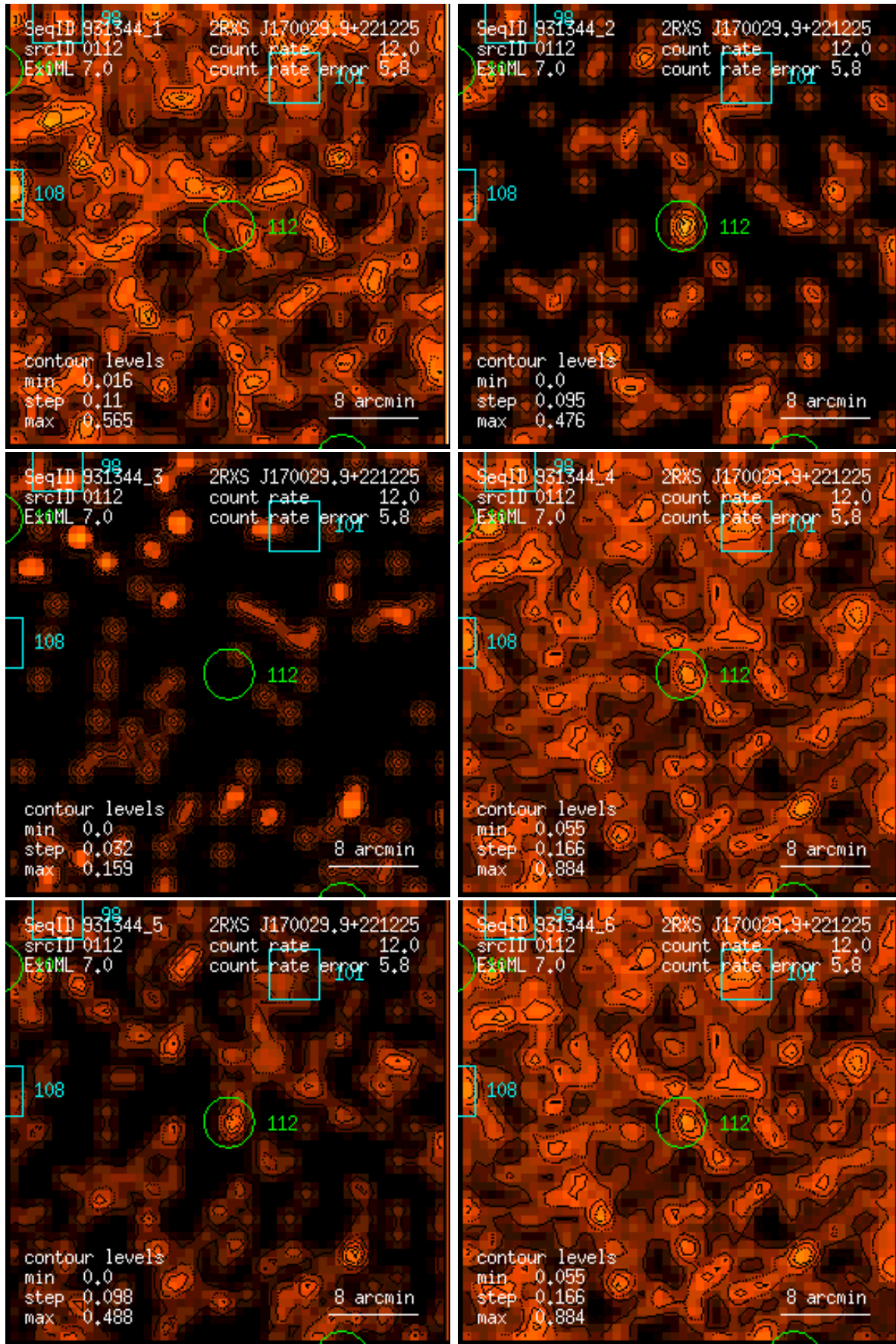
Figure 112: RASS 931344: detection 0112: band rate images, Gaussian filter: (1) PSPC channels 11 – 41, (2) 52 – 90, (3) 91 – 201, (4) 11 – 235, (5) 52 – 201, (6) 11 – 201. Broad band rates in counts/ks. Band rate contour levels in counts/ks/arcmin 2 .
