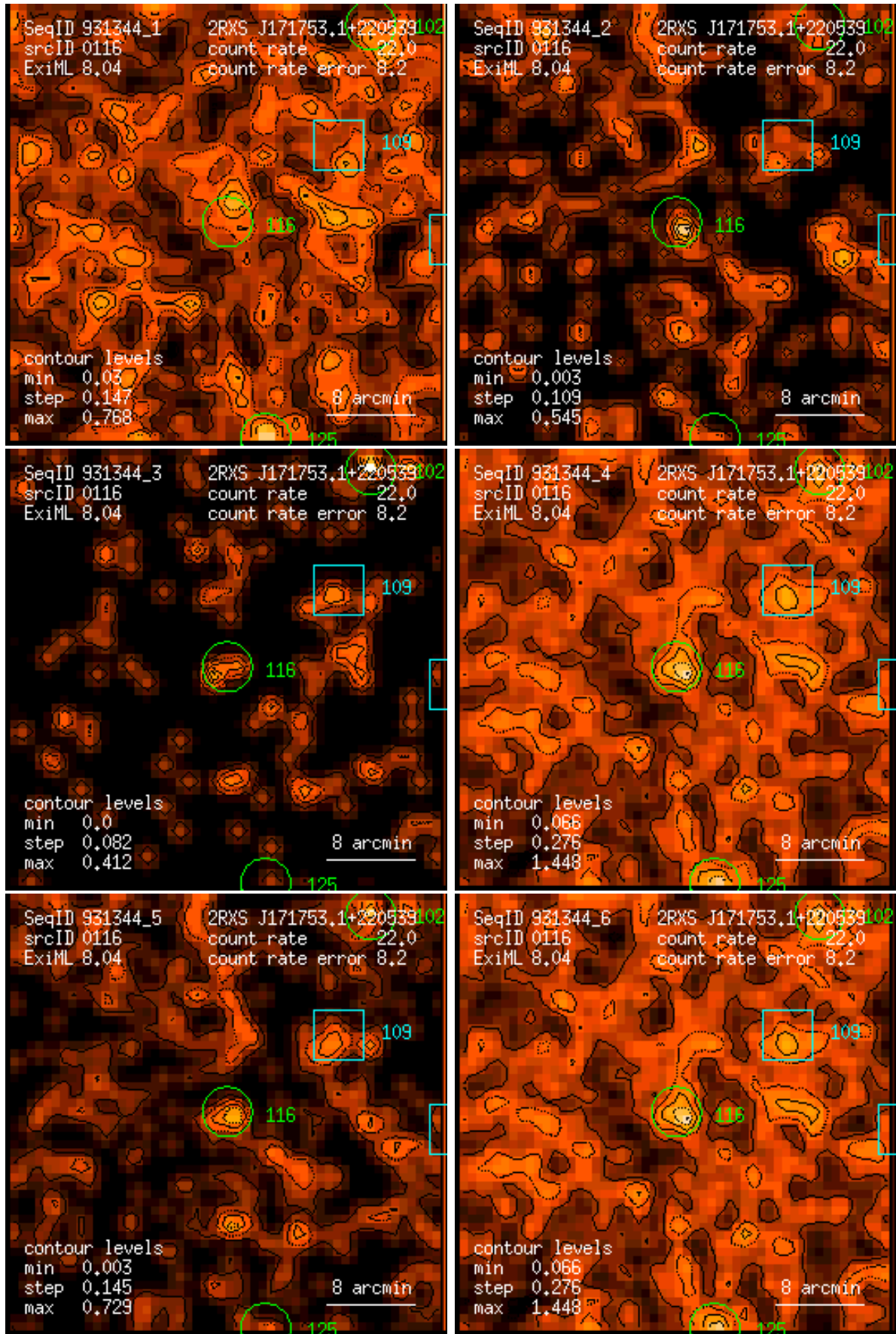
Figure 116: RASS 931344: detection 0116: band rate images, Gaussian filter: (1) PSPC channels 11 – 41, (2) 52 – 90, (3) 91 – 201, (4) 11 – 235, (5) 52 – 201, (6) 11 – 201. Broad band rates in counts/ks. Band rate contour levels in counts/ks/arcmin 2 .
