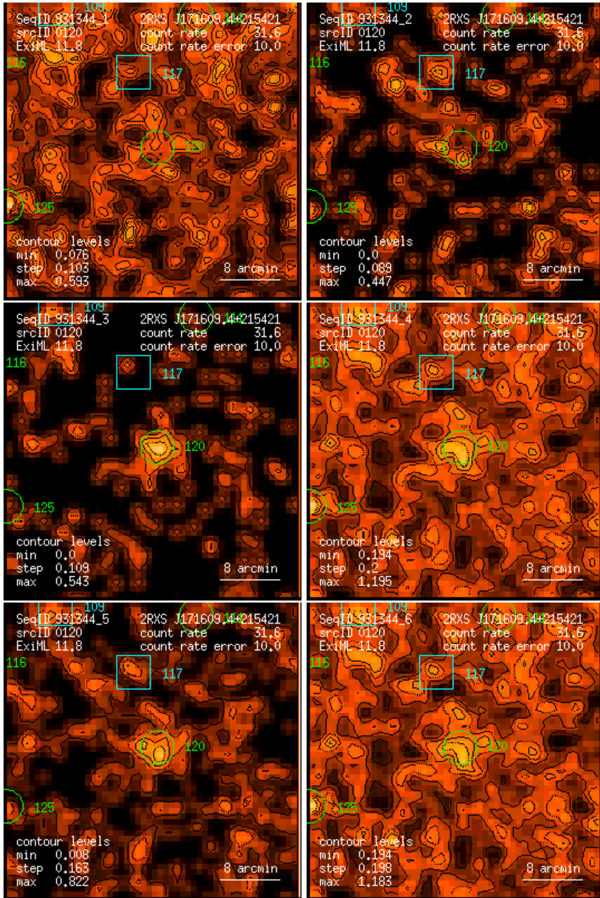
Figure 120: RASS 931344: detection 0120: band rate images, Gaussian filter: (1) PSPC channels 11 – 41, (2) 52 – 90, (3) 91 – 201, (4) 11 – 235, (5) 52 – 201, (6) 11 – 201. Broad band rates in counts/ks. Band rate contour levels in counts/ks/arcmin 2 .
