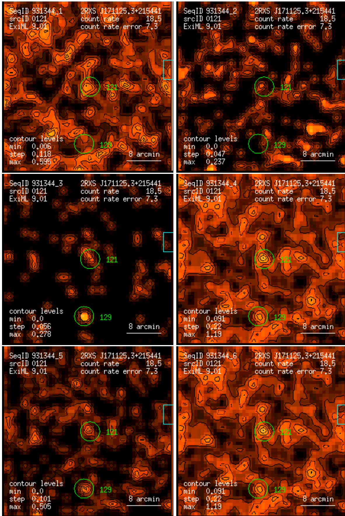
Figure 121: RASS 931344: detection 0121: band rate images, Gaussian filter: (1) PSPC channels 11 – 41, (2) 52 – 90, (3) 91 – 201, (4) 11 – 235, (5) 52 – 201, (6) 11 – 201. Broad band rates in counts/ks. Band rate contour levels in counts/ks/arcmin 2 .
