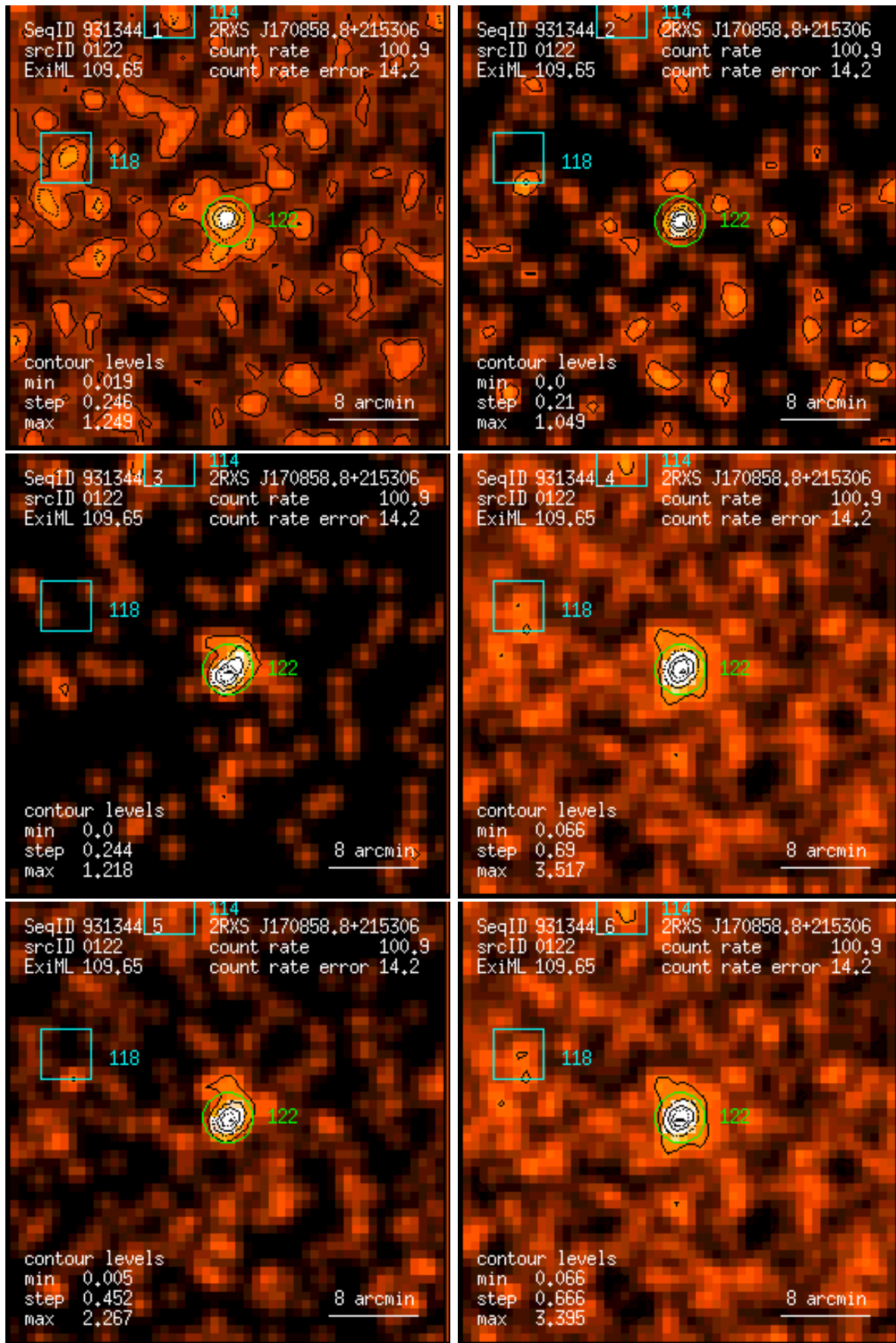
Figure 122: RASS 931344: detection 0122: band rate images, Gaussian filter: (1) PSPC channels 11 – 41, (2) 52 – 90, (3) 91 – 201, (4) 11 – 235, (5) 52 – 201, (6) 11 – 201. Broad band rates in counts/ks. Band rate contour levels in counts/ks/arcmin 2 .
