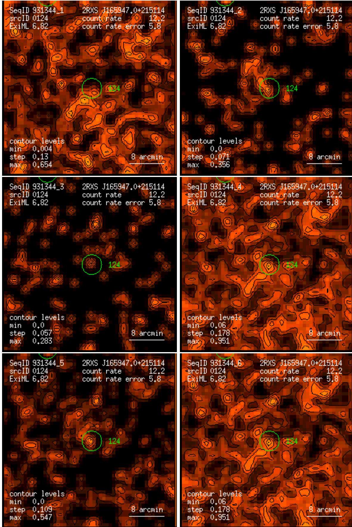
Figure 124: RASS 931344: detection 0124: band rate images, Gaussian filter: (1) PSPC channels 11 – 41, (2) 52 – 90, (3) 91 – 201, (4) 11 – 235, (5) 52 – 201, (6) 11 – 201. Broad band rates in counts/ks. Band rate contour levels in counts/ks/arcmin 2 .
