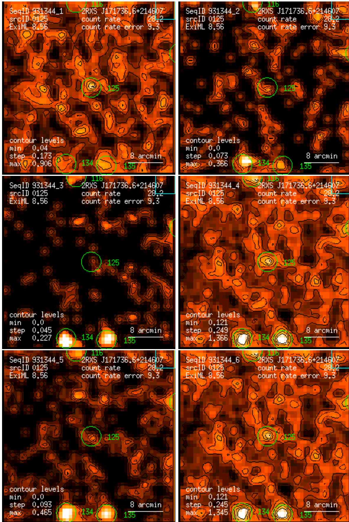
Figure 125: RASS 931344: detection 0125: band rate images, Gaussian filter: (1) PSPC channels 11 – 41, (2) 52 – 90, (3) 91 – 201, (4) 11 – 235, (5) 52 – 201, (6) 11 – 201. Broad band rates in counts/ks. Band rate contour levels in counts/ks/arcmin 2 .
