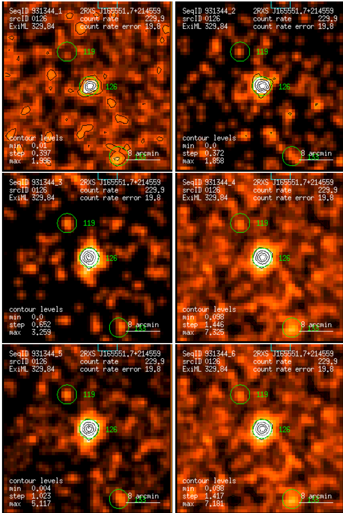
Figure 126: RASS 931344: detection 0126: band rate images, Gaussian filter: (1) PSPC channels 11 – 41, (2) 52 – 90, (3) 91 – 201, (4) 11 – 235, (5) 52 – 201, (6) 11 – 201. Broad band rates in counts/ks. Band rate contour levels in counts/ks/arcmin 2 .
