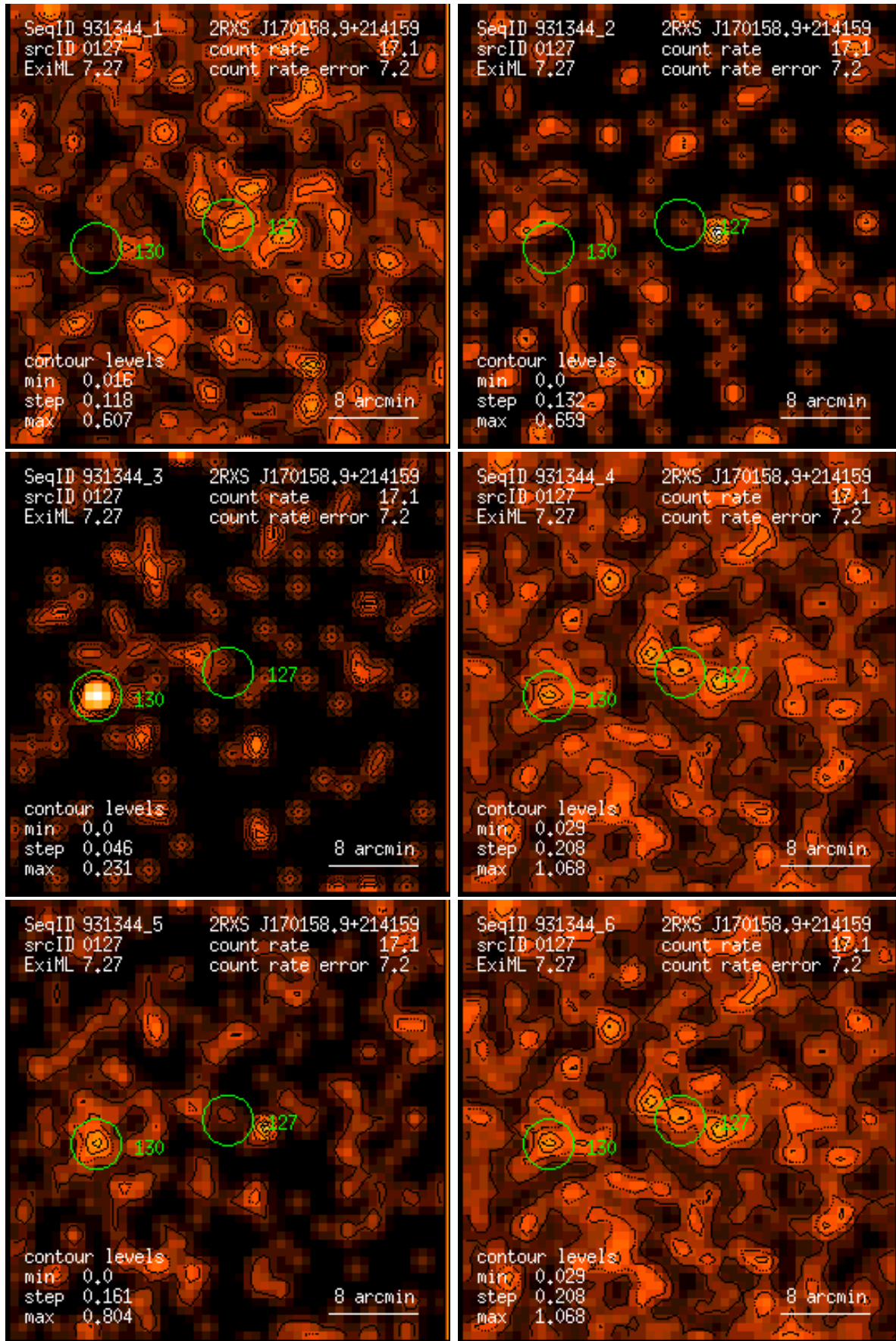
Figure 127: RASS 931344: detection 0127: band rate images, Gaussian filter: (1) PSPC channels 11 – 41, (2) 52 – 90, (3) 91 – 201, (4) 11 – 235, (5) 52 – 201, (6) 11 – 201. Broad band rates in counts/ks. Band rate contour levels in counts/ks/arcmin 2 .
