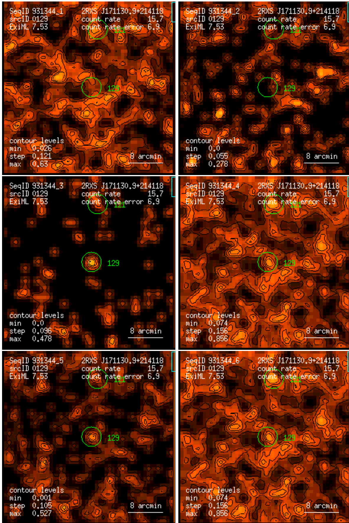
Figure 129: RASS 931344: detection 0129: band rate images, Gaussian filter: (1) PSPC channels 11 – 41, (2) 52 – 90, (3) 91 – 201, (4) 11 – 235, (5) 52 – 201, (6) 11 – 201. Broad band rates in counts/ks. Band rate contour levels in counts/ks/arcmin 2 .
