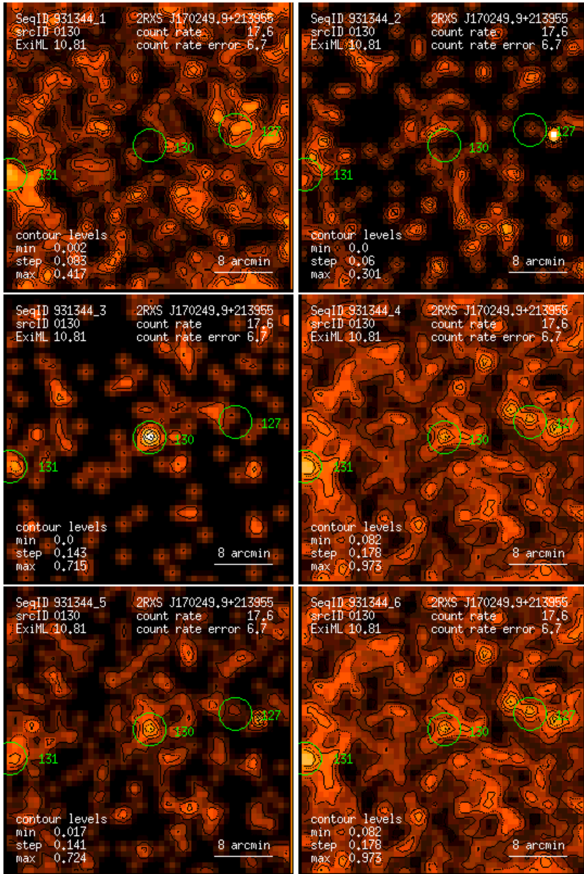
Figure 130: RASS 931344: detection 0130: band rate images, Gaussian filter: (1) PSPC channels 11 – 41, (2) 52 – 90, (3) 91 – 201, (4) 11 – 235, (5) 52 – 201, (6) 11 – 201. Broad band rates in counts/ks. Band rate contour levels in counts/ks/arcmin 2 .
