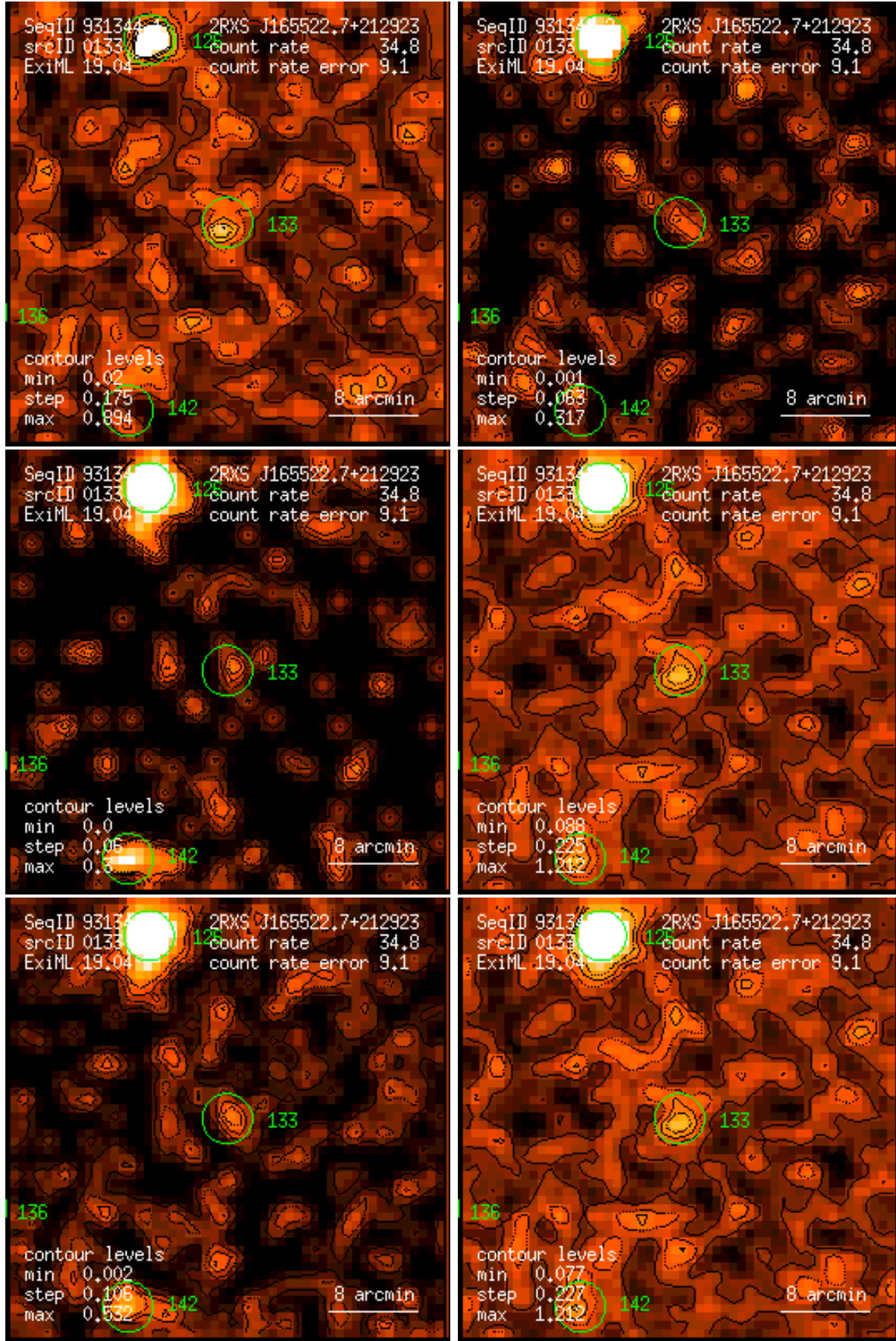
Figure 133: RASS 931344: detection 0133: band rate images, Gaussian filter: (1) PSPC channels 11 – 41, (2) 52 – 90, (3) 91 – 201, (4) 11 – 235, (5) 52 – 201, (6) 11 – 201. Broad band rates in counts/ks. Band rate contour levels in counts/ks/arcmin 2 .
