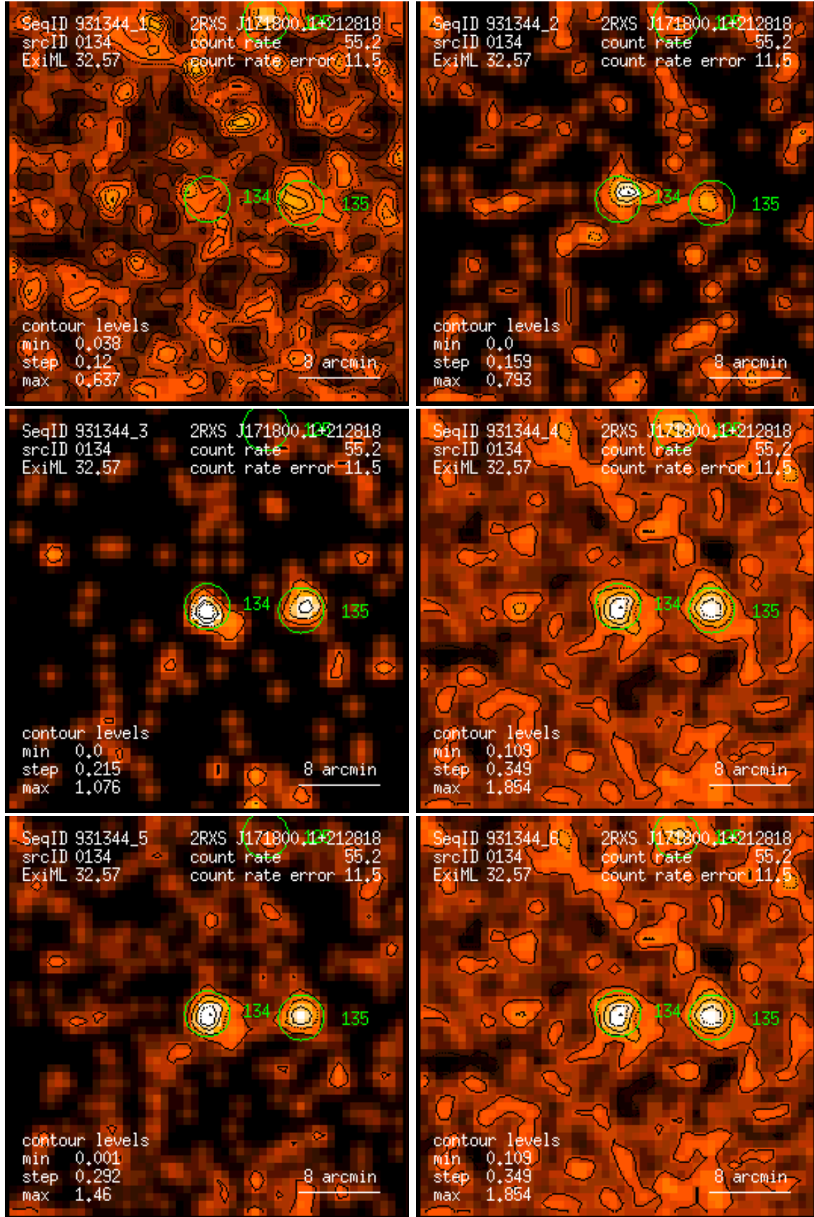
Figure 134: RASS 931344: detection 0134: band rate images, Gaussian filter: (1) PSPC channels 11 – 41, (2) 52 – 90, (3) 91 – 201, (4) 11 – 235, (5) 52 – 201, (6) 11 – 201. Broad band rates in counts/ks. Band rate contour levels in counts/ks/arcmin 2 .
