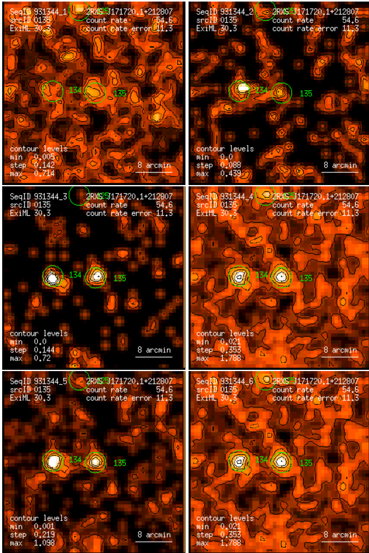
Figure 135: RASS 931344: detection 0135: band rate images, Gaussian filter: (1) PSPC channels 11 – 41, (2) 52 – 90, (3) 91 – 201, (4) 11 – 235, (5) 52 – 201, (6) 11 – 201. Broad band rates in counts/ks. Band rate contour levels in counts/ks/arcmin 2 .
