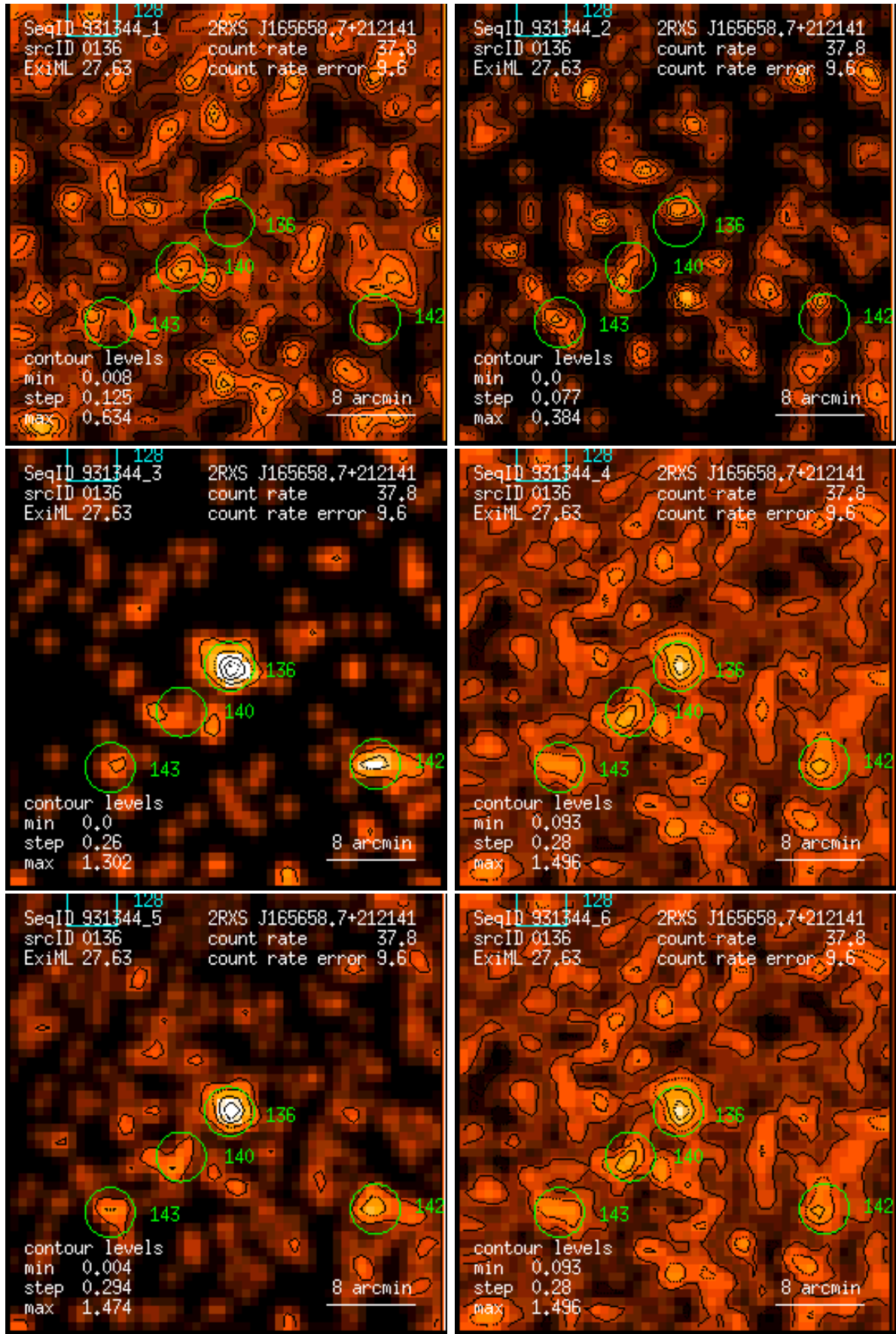
Figure 136: RASS 931344: detection 0136: band rate images, Gaussian filter: (1) PSPC channels 11 – 41, (2) 52 – 90, (3) 91 – 201, (4) 11 – 235, (5) 52 – 201, (6) 11 – 201. Broad band rates in counts/ks. Band rate contour levels in counts/ks/arcmin 2 .
