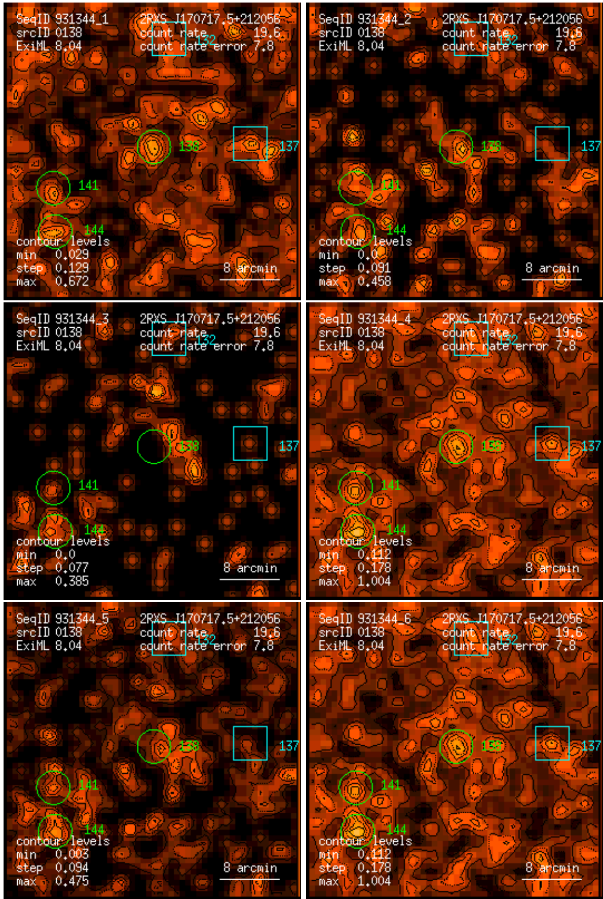
Figure 138: RASS 931344: detection 0138: band rate images, Gaussian filter: (1) PSPC channels 11 – 41, (2) 52 – 90, (3) 91 – 201, (4) 11 – 235, (5) 52 – 201, (6) 11 – 201. Broad band rates in counts/ks. Band rate contour levels in counts/ks/arcmin 2 .
