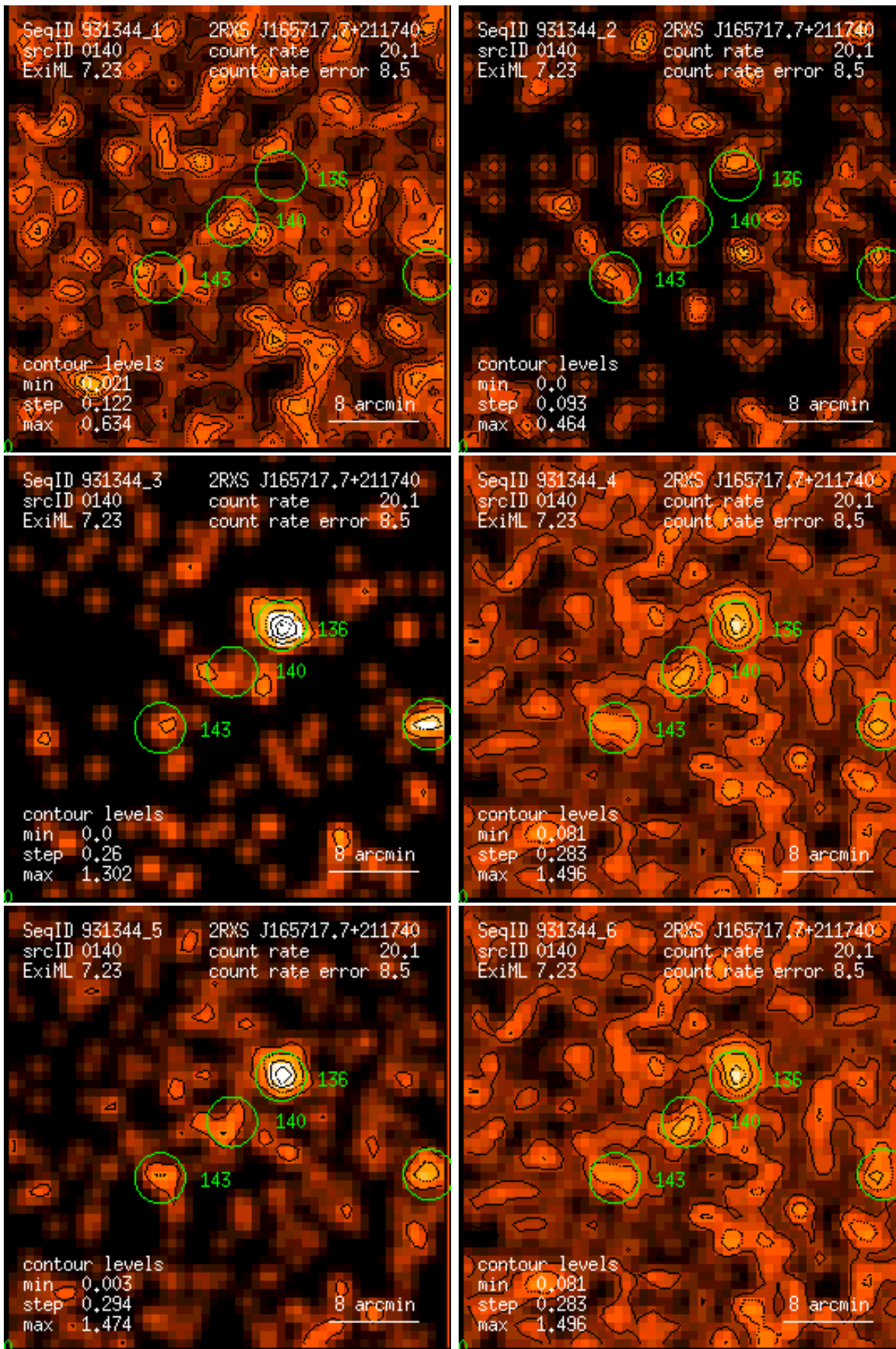
Figure 140: RASS 931344: detection 0140: band rate images, Gaussian filter: (1) PSPC channels 11 – 41, (2) 52 – 90, (3) 91 – 201, (4) 11 – 235, (5) 52 – 201, (6) 11 – 201. Broad band rates in counts/ks. Band rate contour levels in counts/ks/arcmin 2 .
