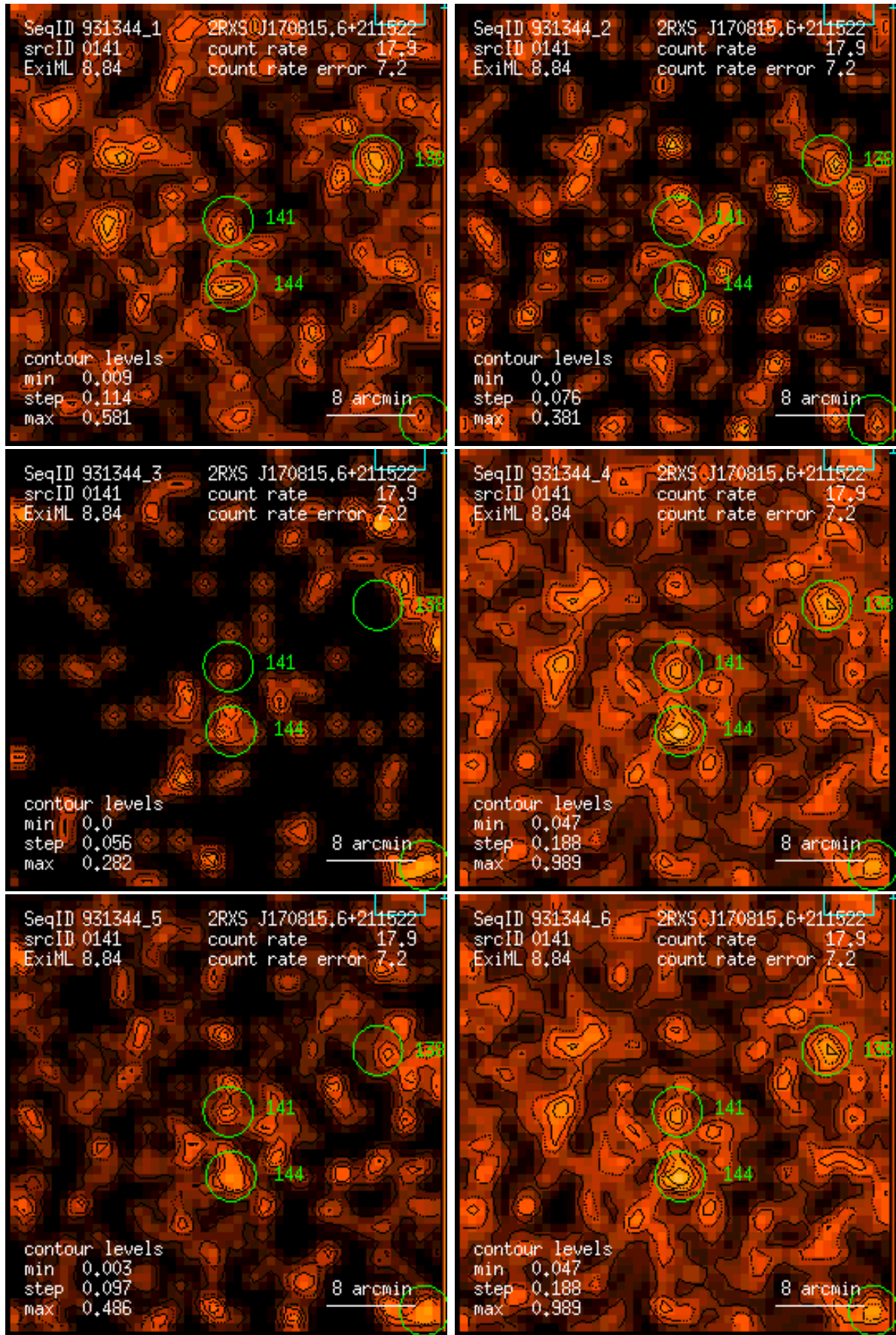
Figure 141: RASS 931344: detection 0141: band rate images, Gaussian filter: (1) PSPC channels 11 – 41, (2) 52 – 90, (3) 91 – 201, (4) 11 – 235, (5) 52 – 201, (6) 11 – 201. Broad band rates in counts/ks. Band rate contour levels in counts/ks/arcmin 2 .
