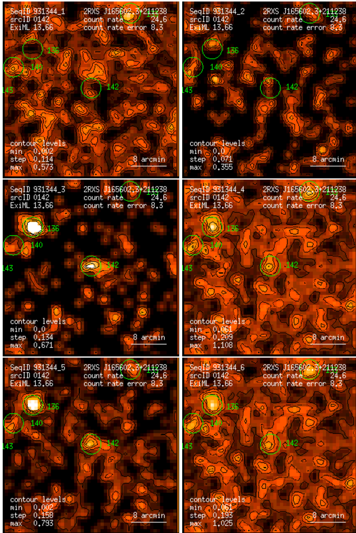
Figure 142: RASS 931344: detection 0142: band rate images, Gaussian filter: (1) PSPC channels 11 – 41, (2) 52 – 90, (3) 91 – 201, (4) 11 – 235, (5) 52 – 201, (6) 11 – 201. Broad band rates in counts/ks. Band rate contour levels in counts/ks/arcmin 2 .
