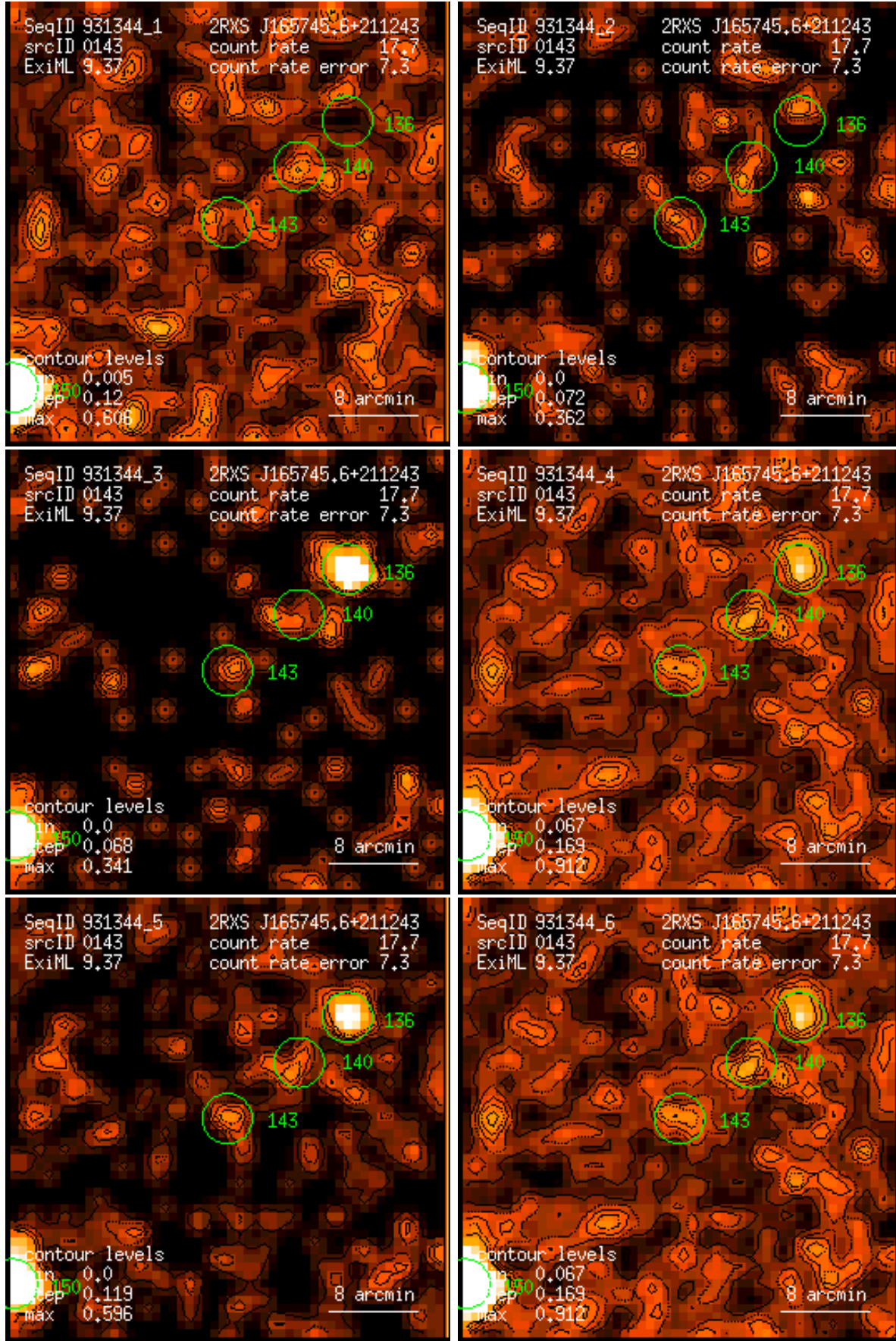
Figure 143: RASS 931344: detection 0143: band rate images, Gaussian filter: (1) PSPC channels 11 – 41, (2) 52 – 90, (3) 91 – 201, (4) 11 – 235, (5) 52 – 201, (6) 11 – 201. Broad band rates in counts/ks. Band rate contour levels in counts/ks/arcmin 2 .
