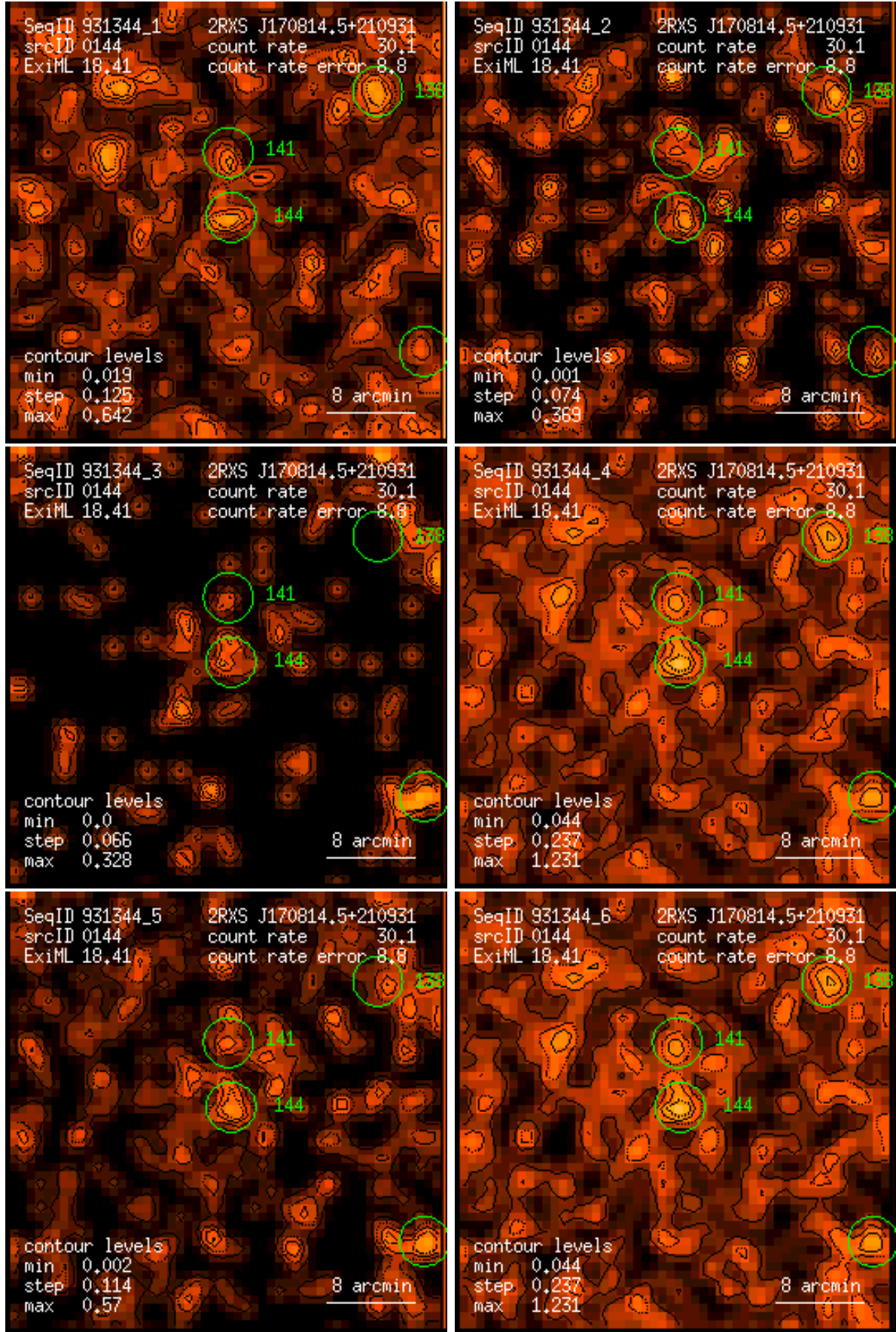
Figure 144: RASS 931344: detection 0144: band rate images, Gaussian filter: (1) PSPC channels 11 – 41, (2) 52 – 90, (3) 91 – 201, (4) 11 – 235, (5) 52 – 201, (6) 11 – 201. Broad band rates in counts/ks. Band rate contour levels in counts/ks/arcmin 2 .
