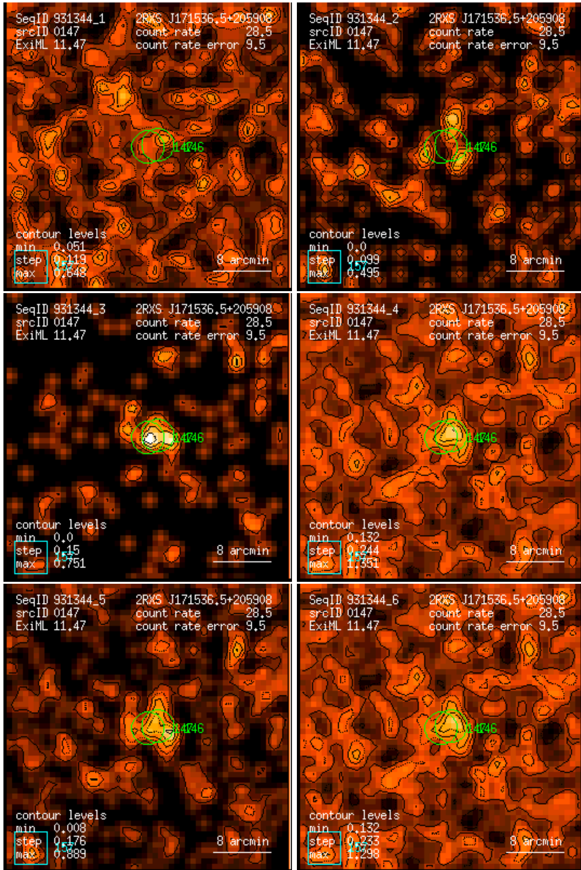
Figure 147: RASS 931344: detection 0147: band rate images, Gaussian filter: (1) PSPC channels 11 – 41, (2) 52 – 90, (3) 91 – 201, (4) 11 – 235, (5) 52 – 201, (6) 11 – 201. Broad band rates in counts/ks. Band rate contour levels in counts/ks/arcmin 2 .
